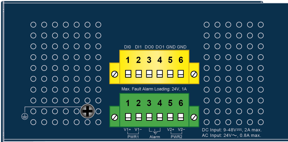
Figure 2-1-4a: Industrial Managed Switch Upper Panel.
