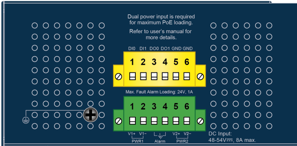
Figure 2-1-4b: Industrial Managed Switch Upper Panel.
