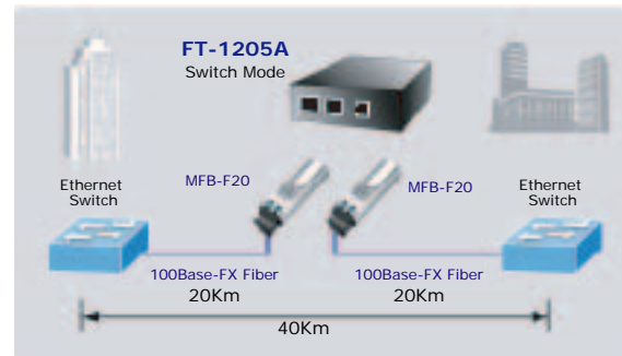
Fiber Switch mode - distance extension
