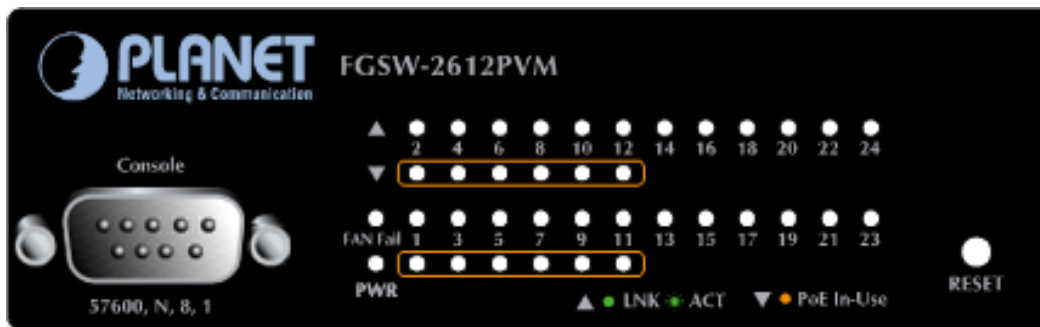
Figure 2-7: FGSW-2612PVM LED panel
