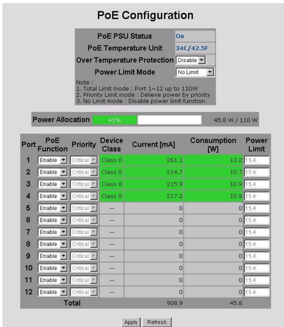
Figure 4-13-1: PoE Configuration
