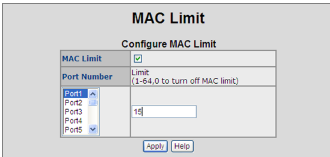
Figure 4-11-1: MAC Limit - Configure MAC Limit
