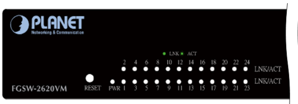
Figure 2-5: FGSW-2620VM LED panel
