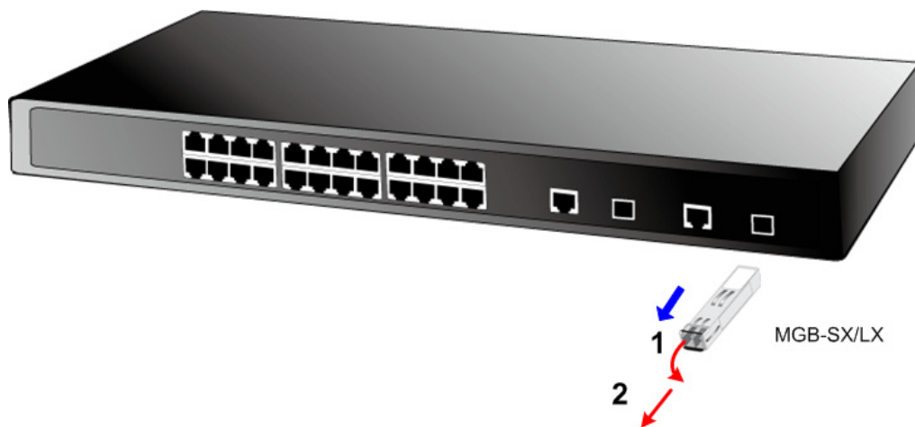
Figure 2-17: Pull out the SFP transceiver
