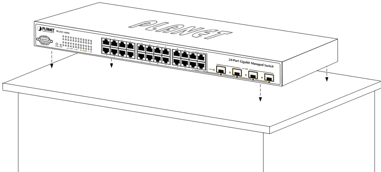
Figure 2-13: Place the Managed Switch on the desktop
