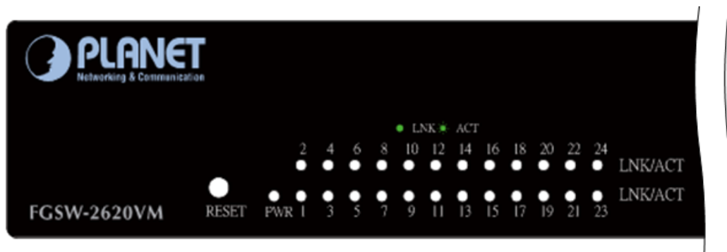
Figure 2-4: FGSW-2620VM LED panel
