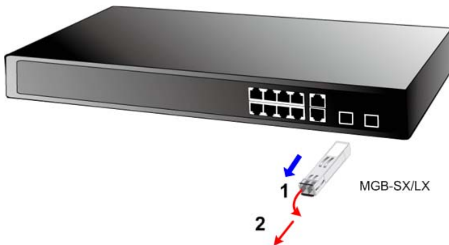
Figure 2-11: Pull out the SFP transceiver
