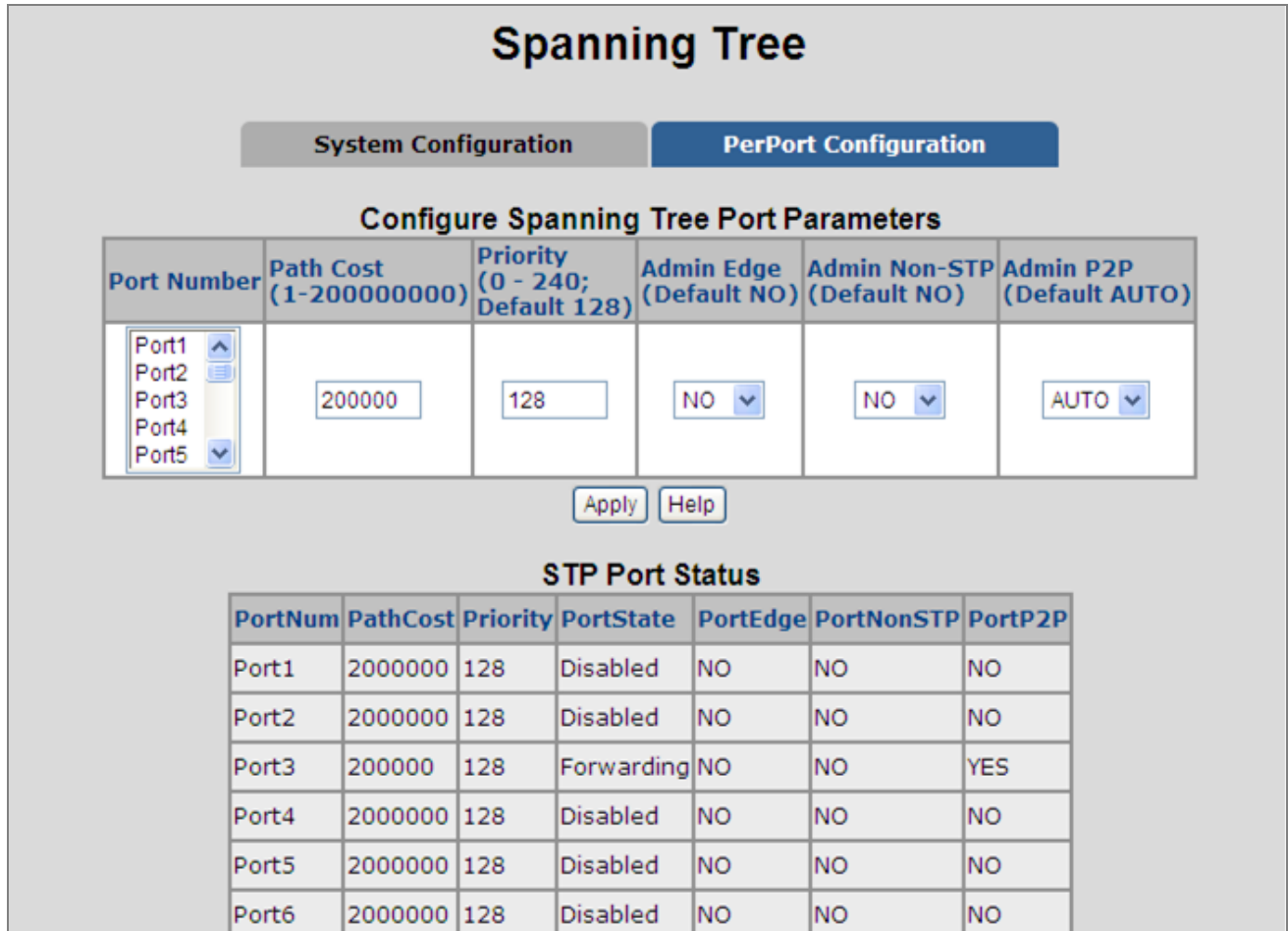
Figure 4-5-6: STP Port Configuration interface
