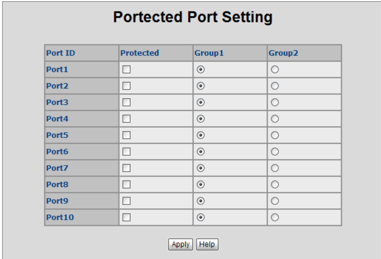
Figure 4-3-6: Protected Port Setting Web interface
