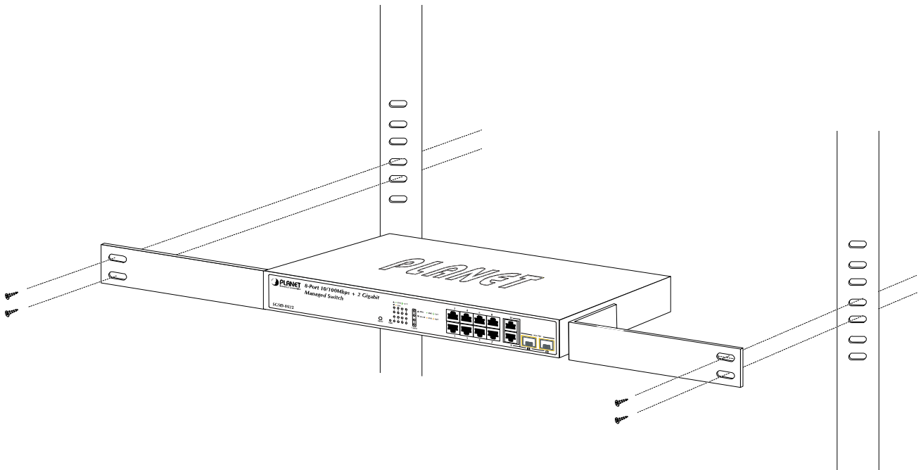
Figure 2-9: Mounting the Switch in a Rack
