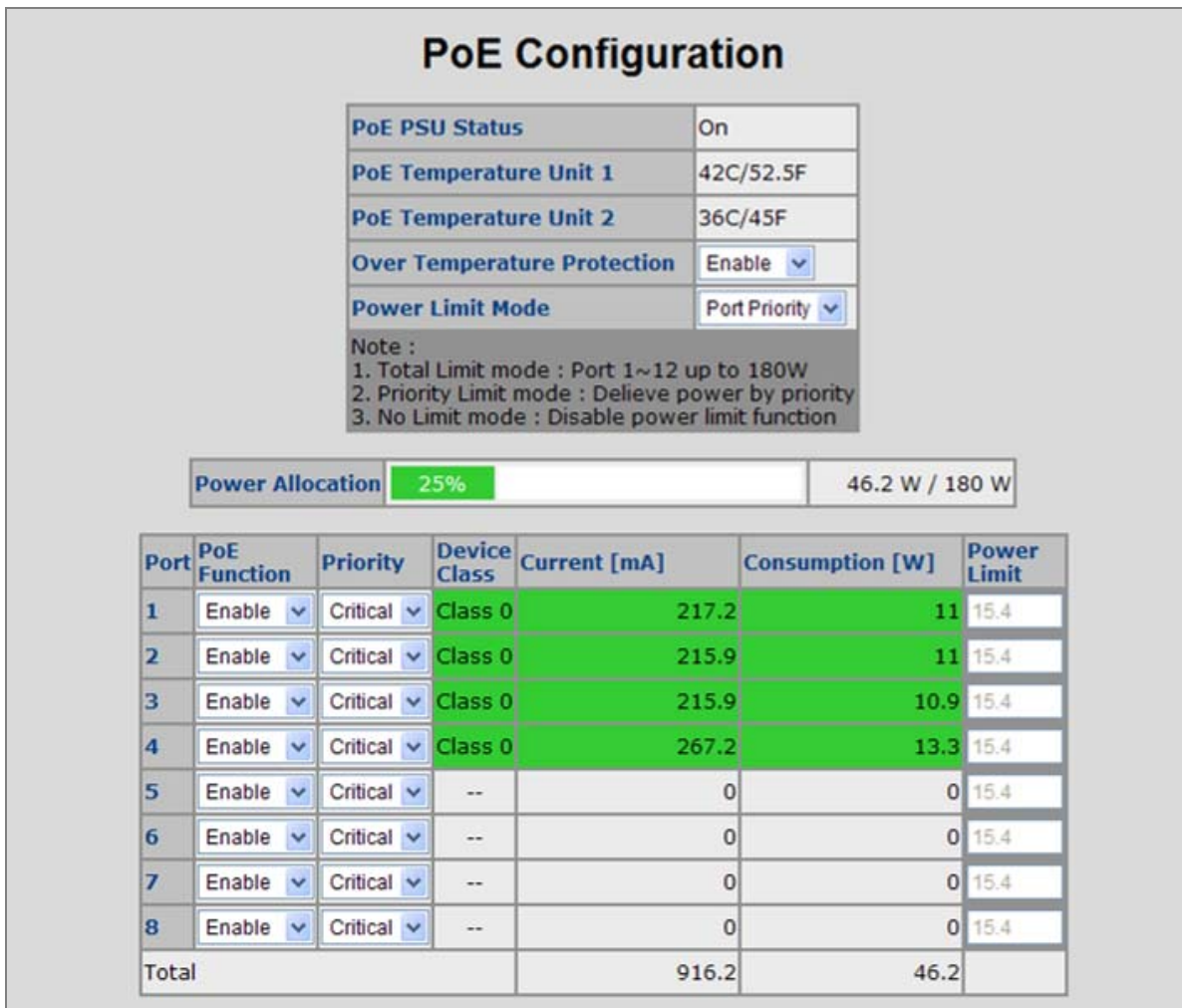
Figure 4-13-1: PoE Configuration
