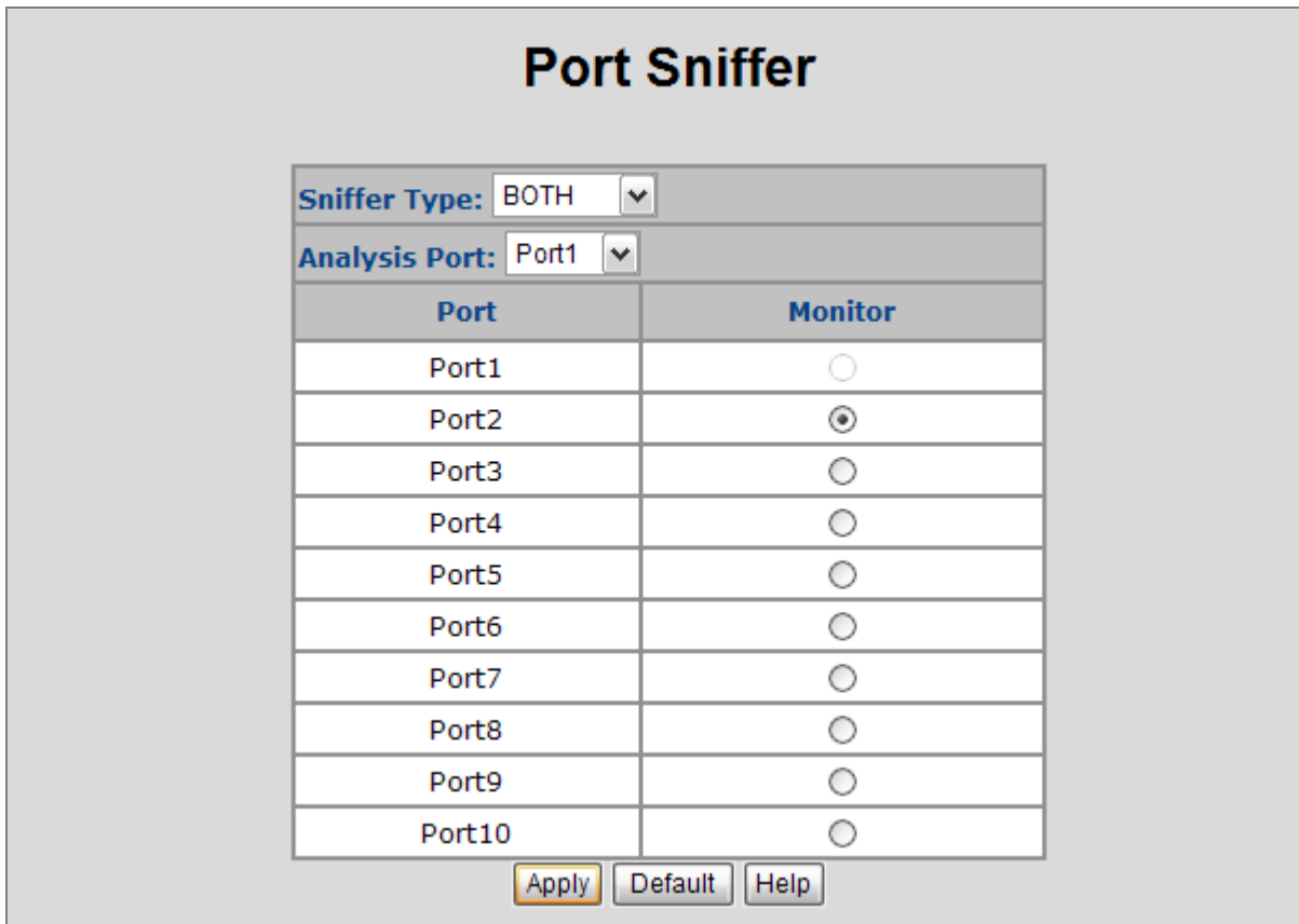
Figure 4-3-5: Port Sniffer interface
