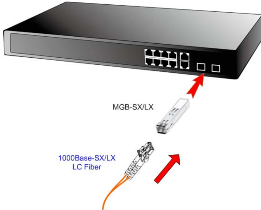
Figure 2-10: Plug-in the SFP transceiver
