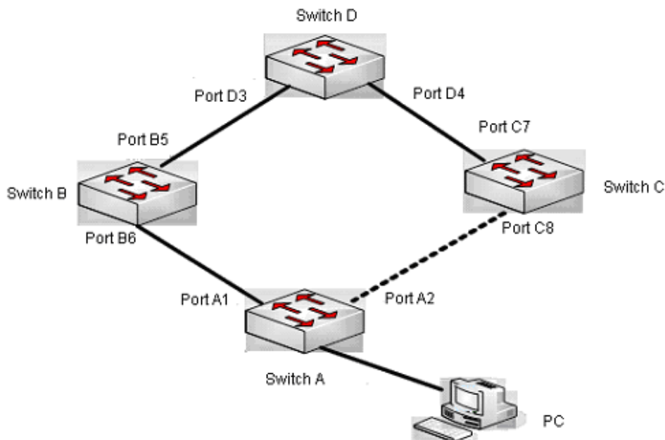
Figure 62-1-1 ULSM using scene
