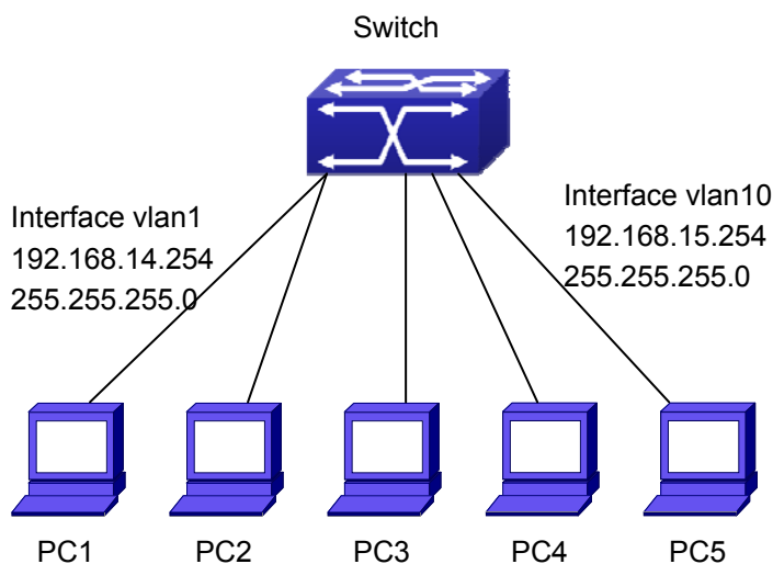
Figure 26-3-1 Gratuitous ARP Configuration Example
