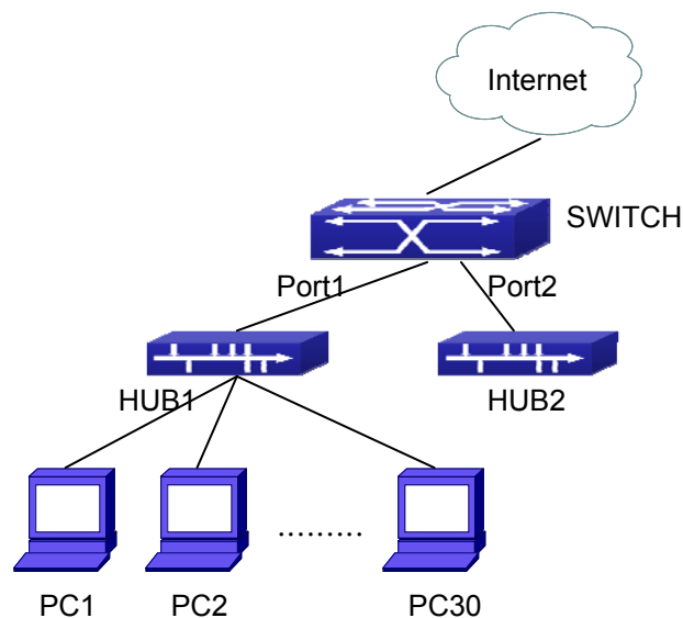
Figure 49-3-1 a typical configuration example of AM function
