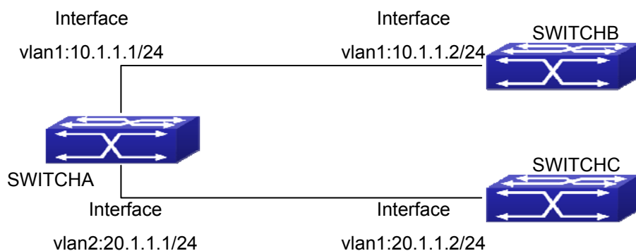
Figure 35-3-1 RIP example
