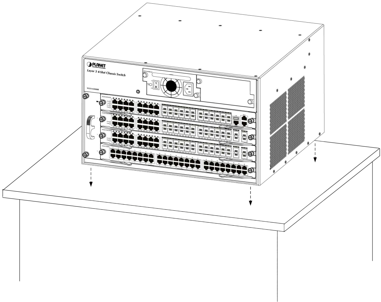
Figure 2-2-1 Place the Chassis Switch on the desktop
