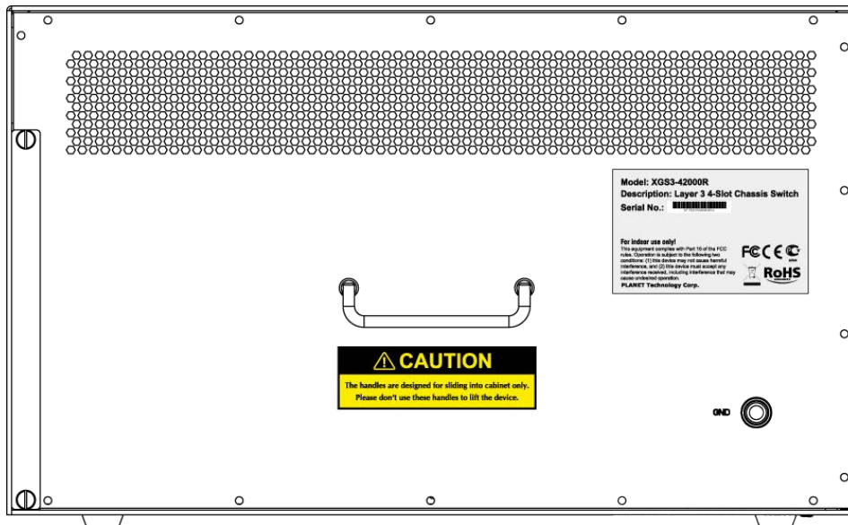
Figure 2-1-2 XGS3-42000R rear panel
