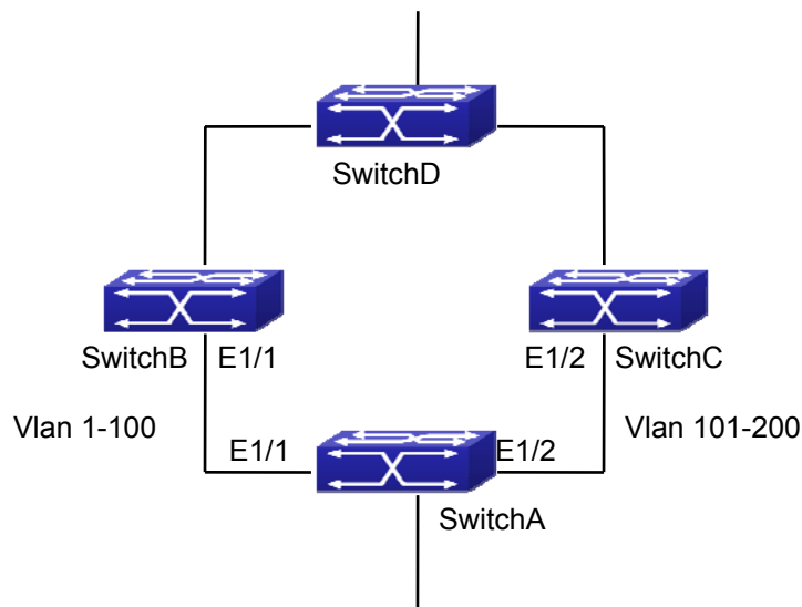
Figure 61-3-2 ULPP typical example2
