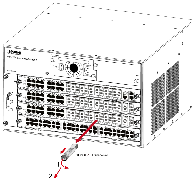
Figure 2-2-11 Pull out the SFP/SFP+ transceiver
