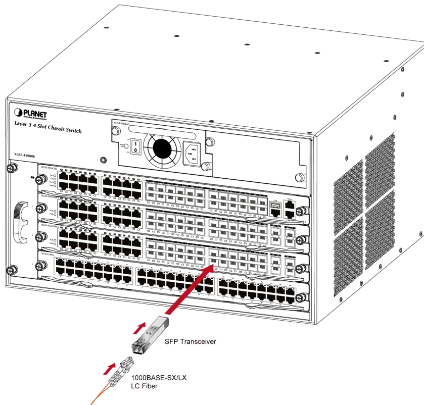
Figure 2-2-9 Plug-in the SFP transceiver
