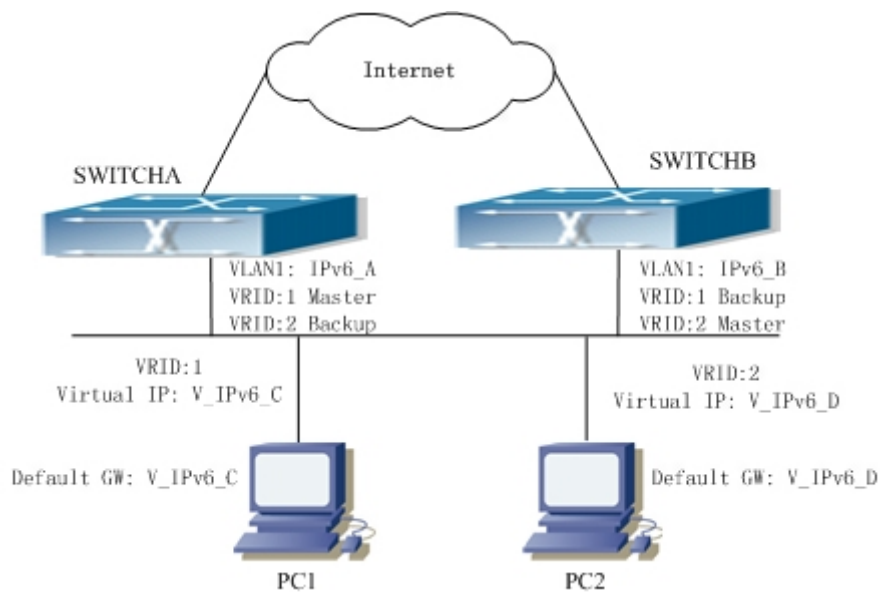
Figure 59-3-1 VRRPv3 Typical Network Topology
