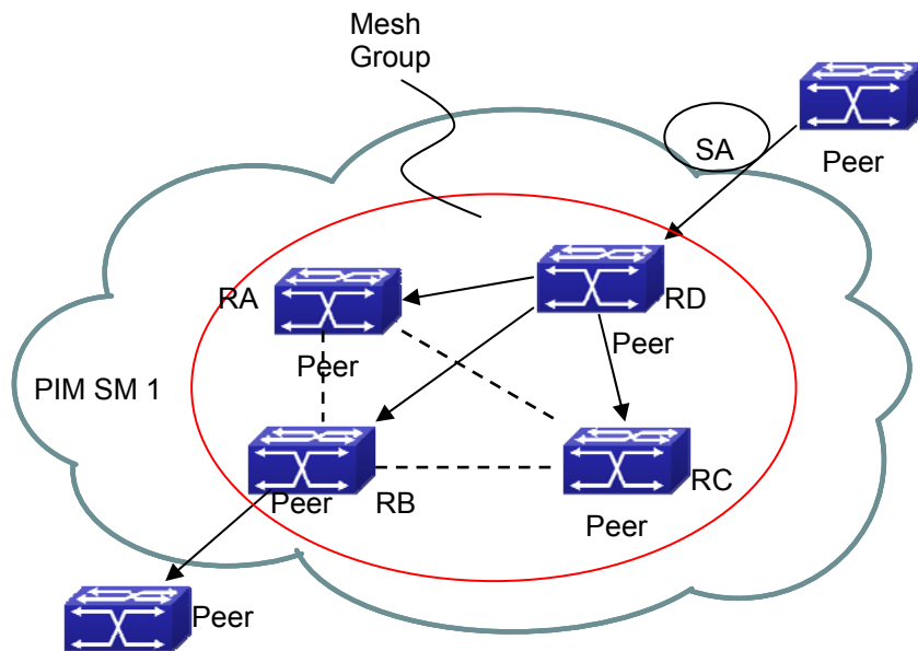
Figure 43-4-3 Flooding of SA messages with mesh group configuration
