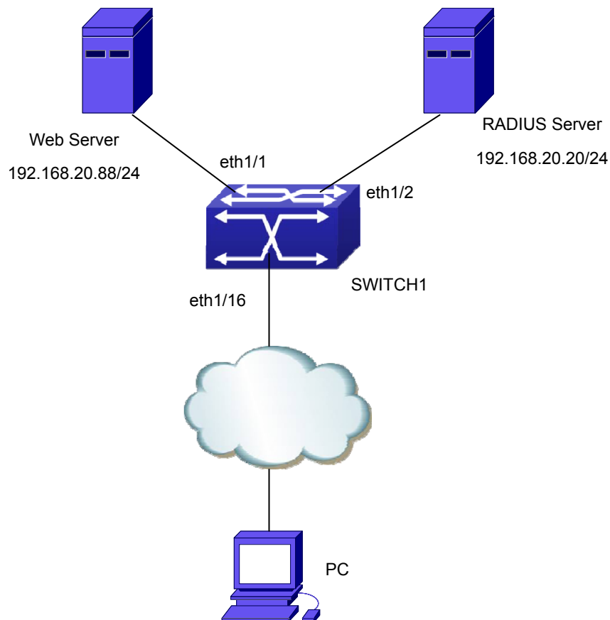
Figure 47-3-5 802.1x Web Proxy Authentication
