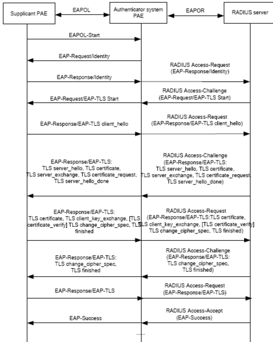
Figure 47-1-10 the Authentication Flow of 802.1x EAP-TLS
