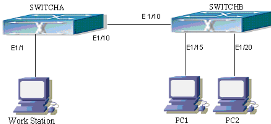
Figure 45-3-1 Function configuration of the Multicast VLAN
