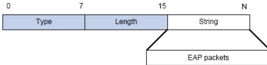
Figure 47-1-6 the Encapsulation of EAP-Message Attribute
