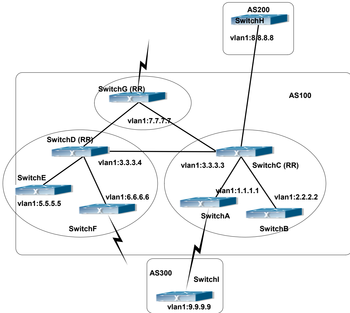
Figure 39-3-3 the Topological Map of Route Reflector
