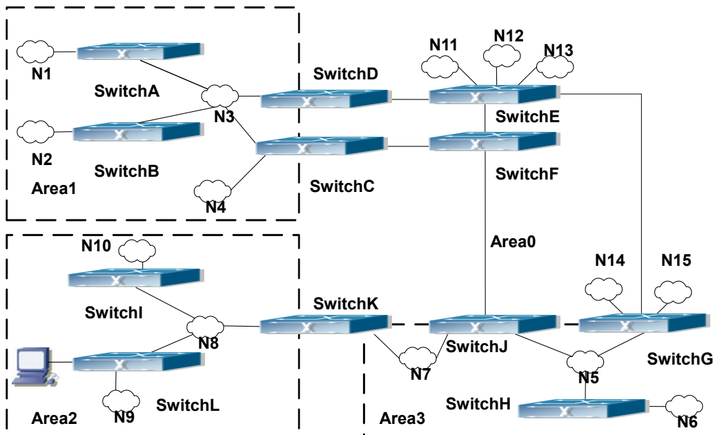
Figure 37-3-2 Typical complex OSPF autonomous system
