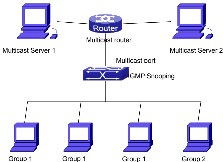
Figure 43-10-1 Enabling IGMP Snooping function
