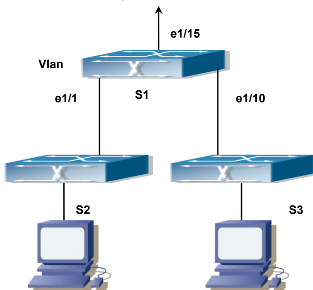
Figure 8-3-1 A typical example of port isolation function
