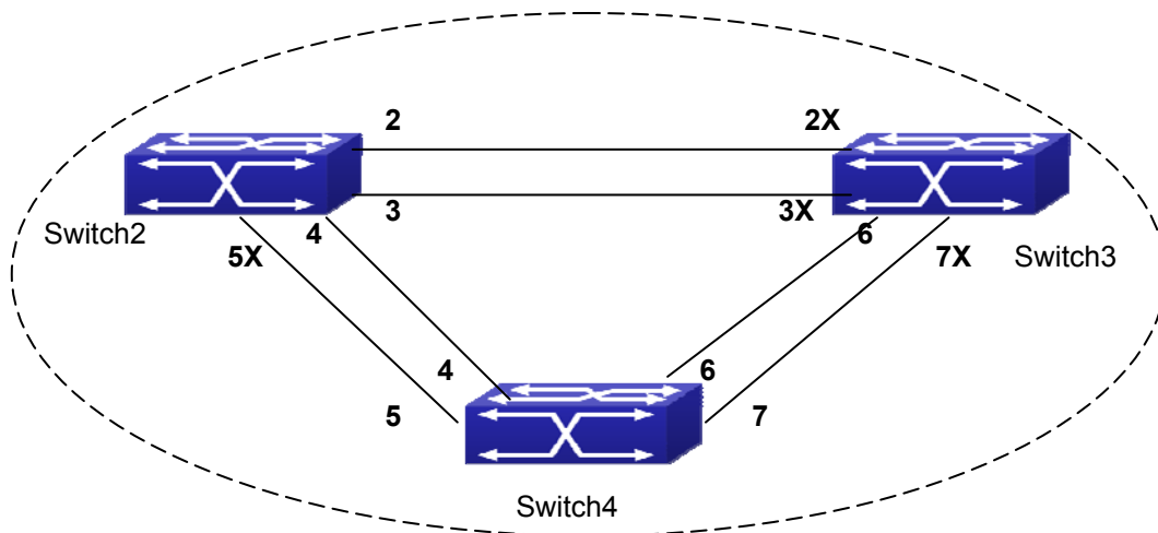
Figure 16-3-4 The Topology Of the Instance 4 after the MSTP Calculation
