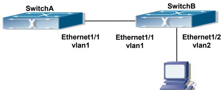
Figure 43-9-1 IGMP Network Topology Diagram
