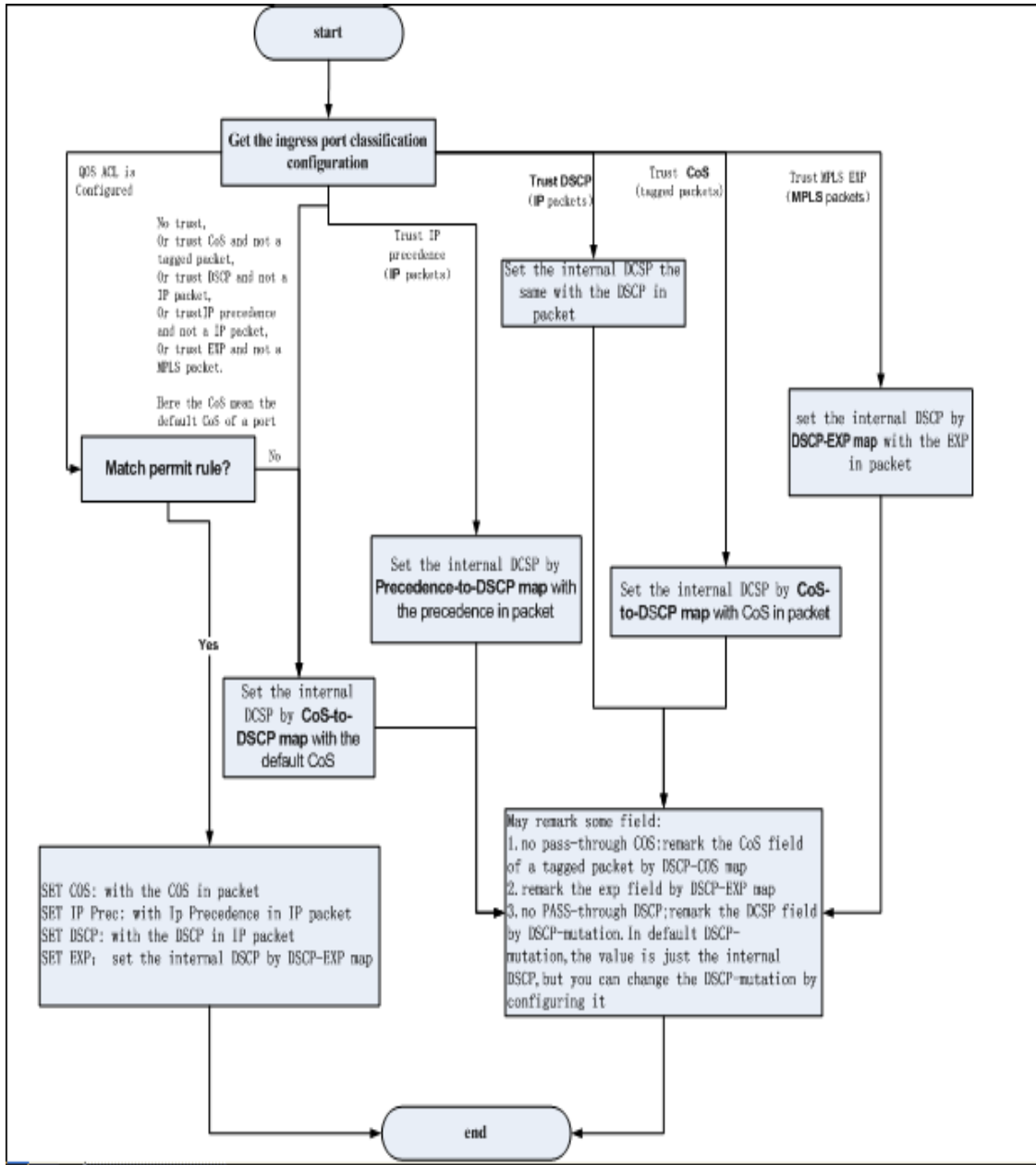
Figure 17-1-4 Classification process
