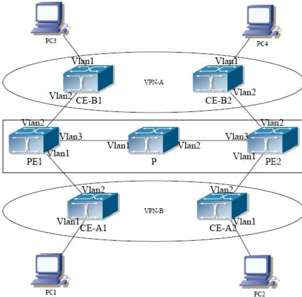
Figure 39-3-5 Example of MPLS VPN
