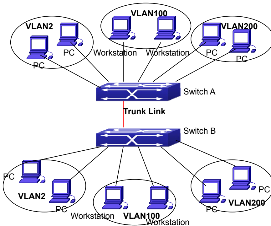
Figure 14-1-2 Typical VLAN Application Topology
