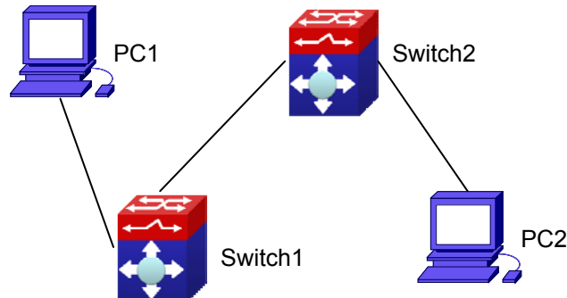
Figure 21-2-1 IPv4 configuration example
