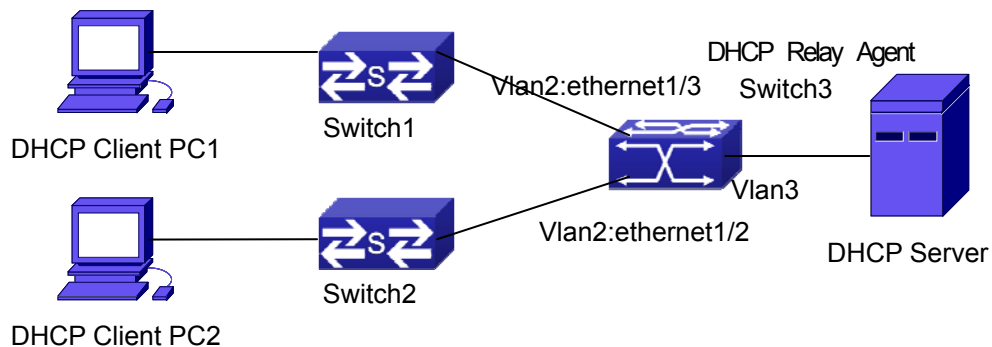
Figure 30-3-1 A DHCP option 82 typical application example
