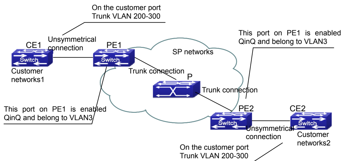
Figure 14-3-1 Dot1q-tunnel based Internetworking mode
