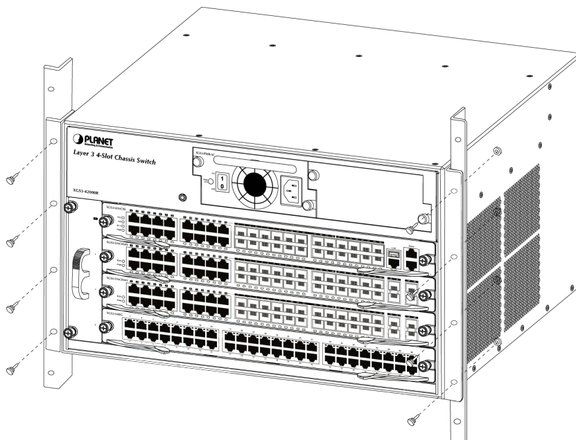
Figure 2-2-3 Mounting Chassis Switch in a Rack
