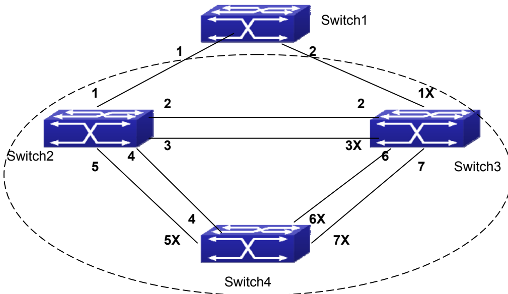
Figure 16-3-2 The Topology Of the Instance 0 after the MSTP Calculation
