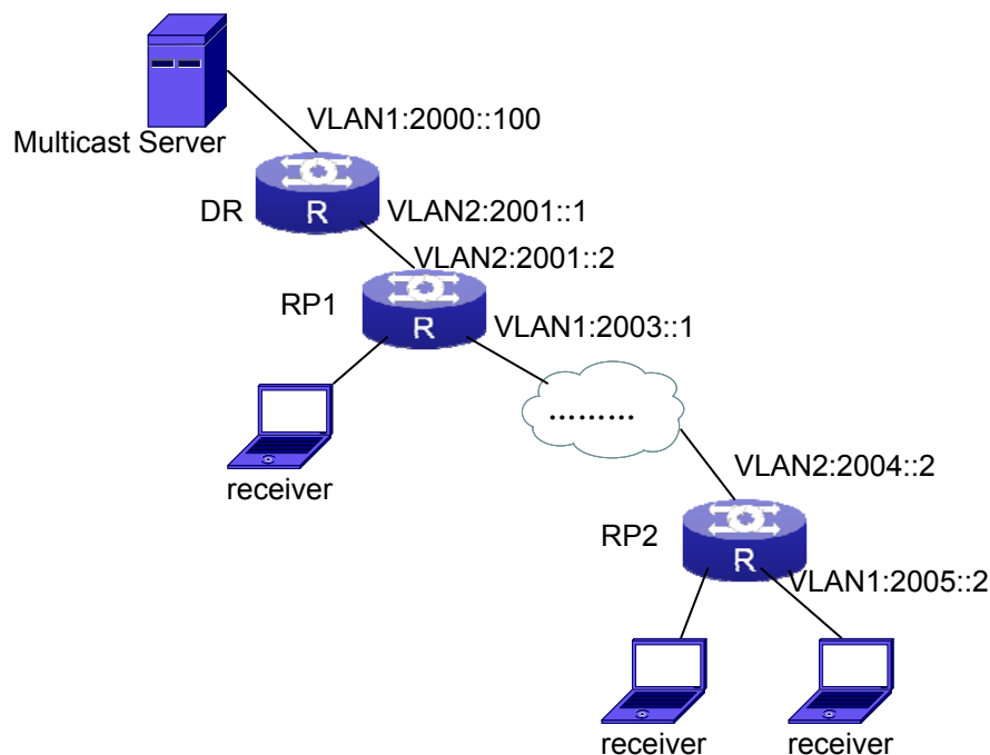
Figure 44-3-1 The ANYCAST RP v6 function of a router
