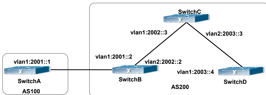
Figure 40-3-1 BGP Network Topological Map
