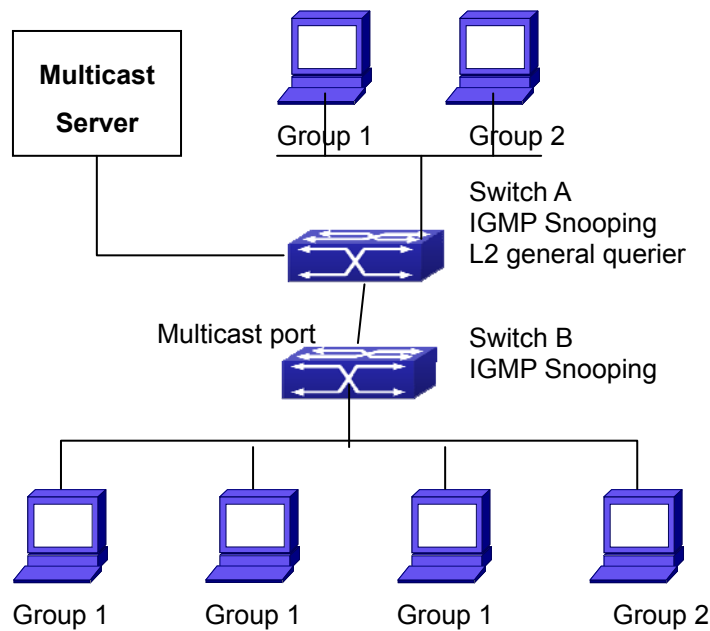
Figure 43-10-1 The switches as IGMP Queries
