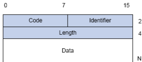
Figure 47-1-4 the Format of EAP Data Packets
