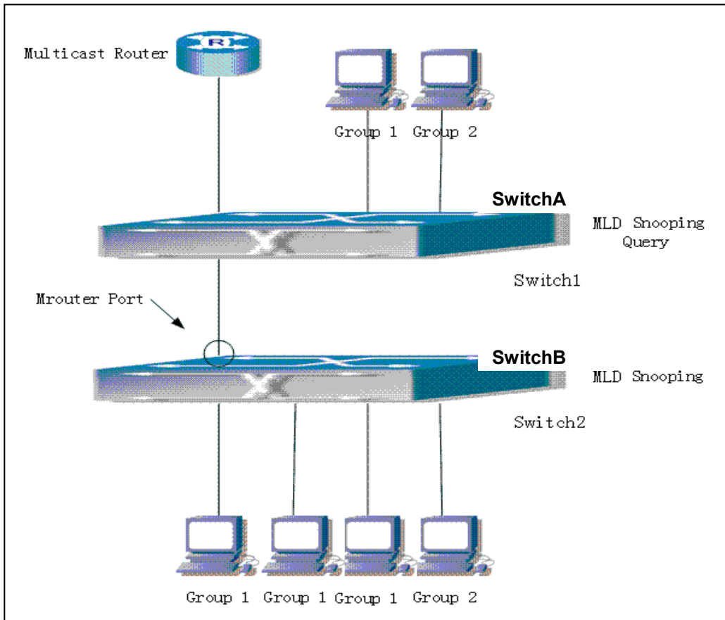
Figure 44-7-2 Switch as MLD Querier Function figure
