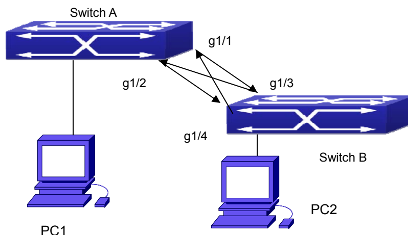
Figure 10-3-1 Fiber Cross Connection
