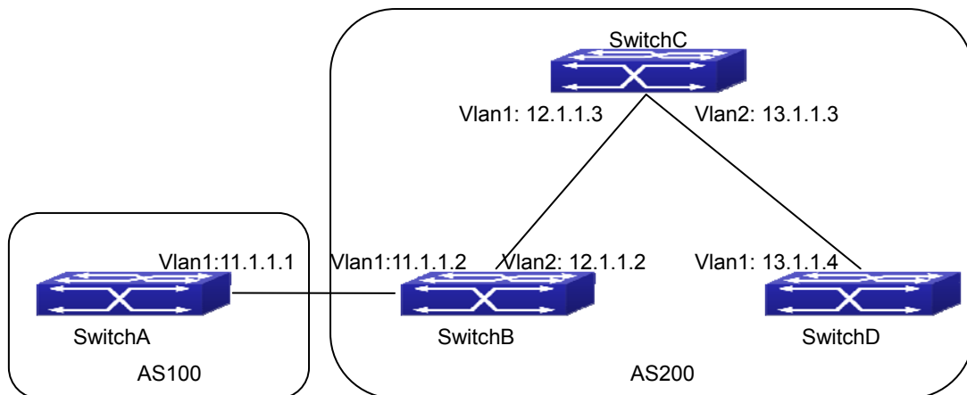
Figure 39-3-1 BGP Network Topological Map
