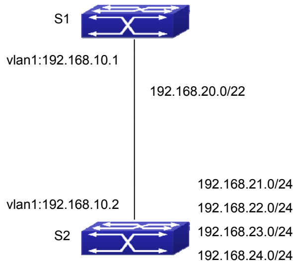
Figure 35-3-2 Typical application of RIP aggregation
