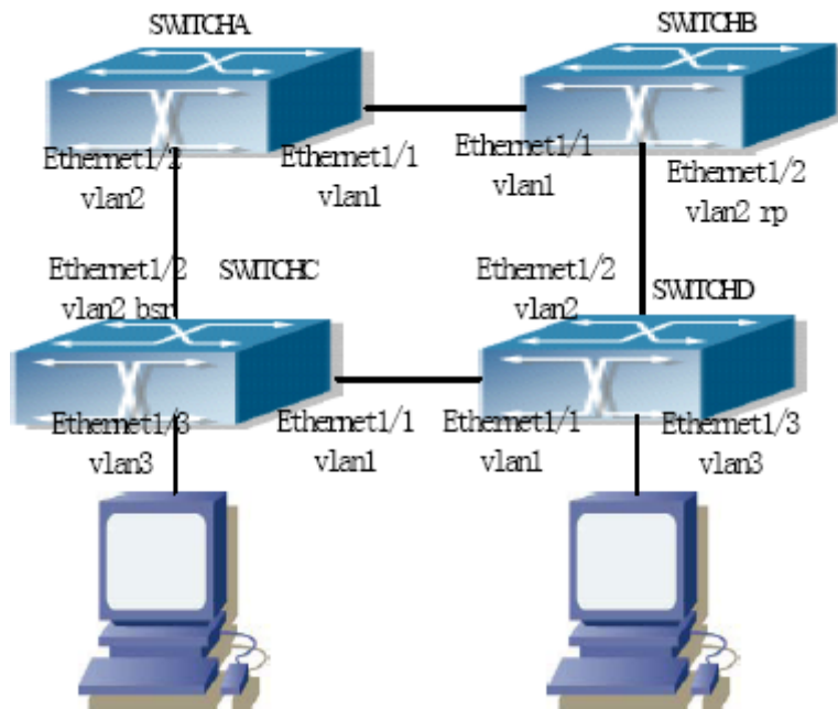
Figure 44-4-1 PIM-SSM typical environment
