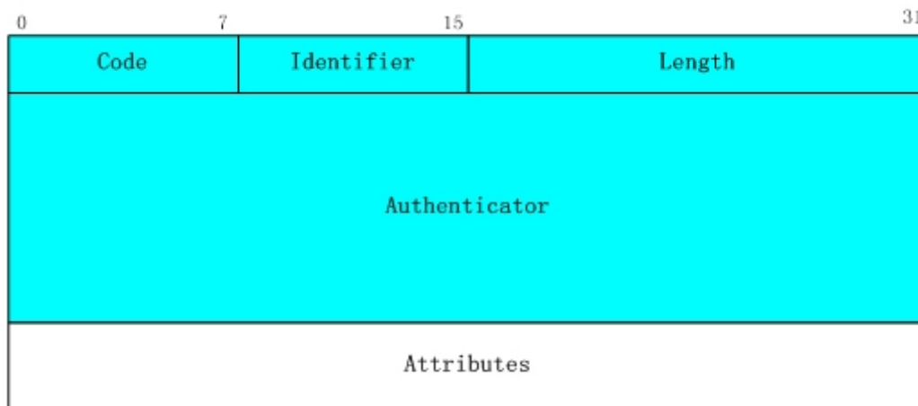
Figure 52-1-1 Message structure for RADIUS
