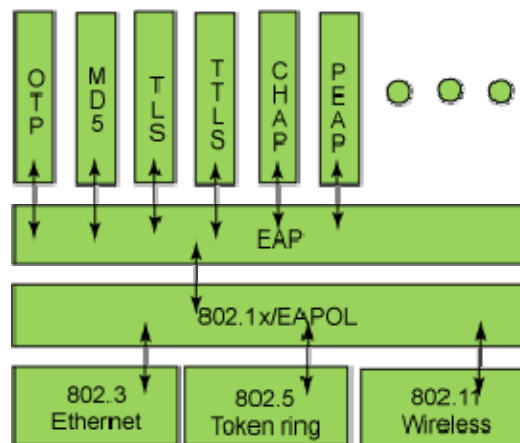
Figure 47-1-8 the Protocol Stack of EAP Authentication Method
