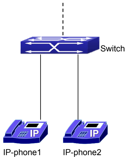
Figure 14-6-1 VLAN typical apply topology
