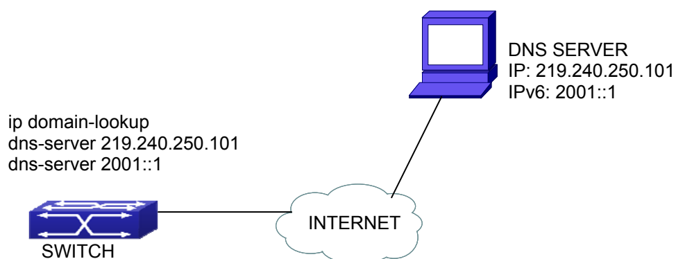
Figure 65-3-1 DNS CLIENT typical environment
