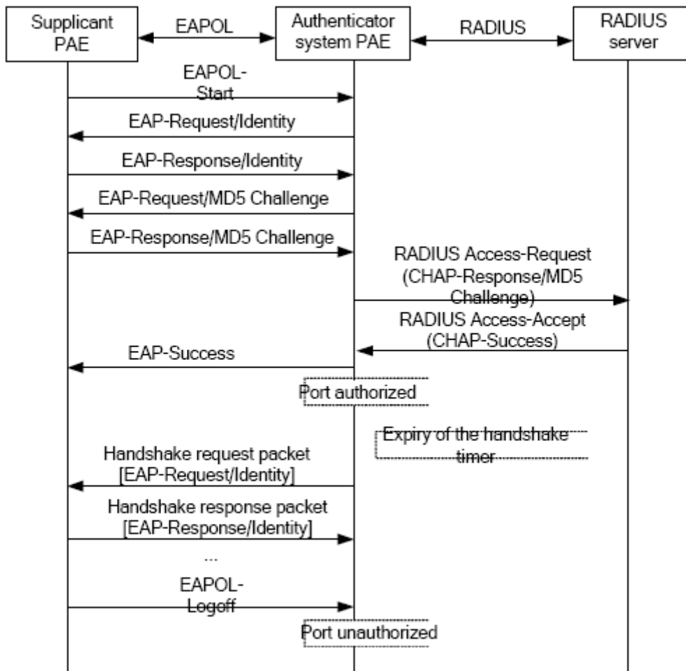
Figure 47-1-12 the Authentication Flow of 802.1x EAP Termination Mode
