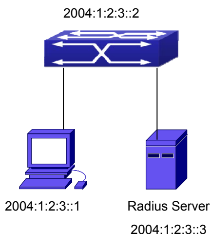
Figure 52-3-2 The Topology of IPv6 Radius configuration
