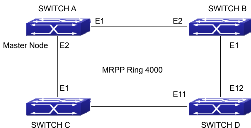
Figure 60-3-1 MRPP typical configuration scenario
