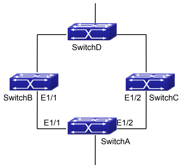
Figure 61-3-1 ULPP typical example1
