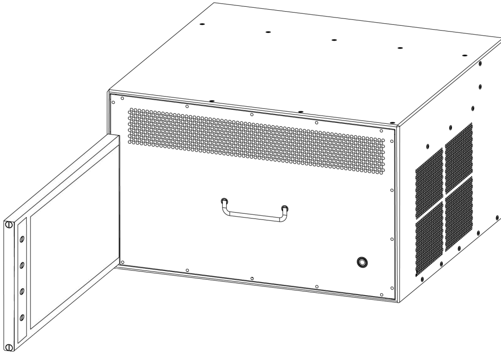
Figure 2-2-6 Installation and Removal of the XGS3-42000R Dust Gauze
