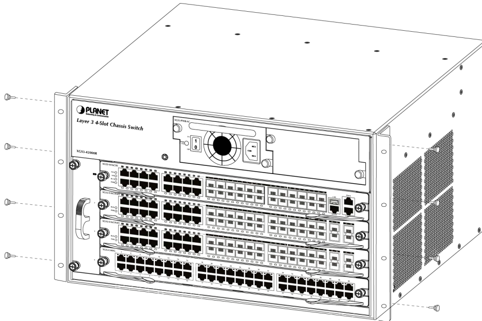
Figure 2-2-2 Attach brackets to the Chassis Switch.
