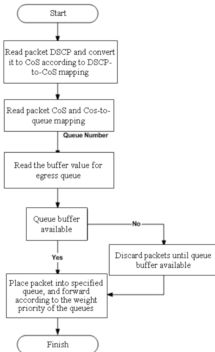
Figure 17-1-6 Queuing and Scheduling process
