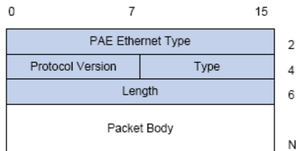
Figure 47-1-3 the Format of EAPOL Data Packet
