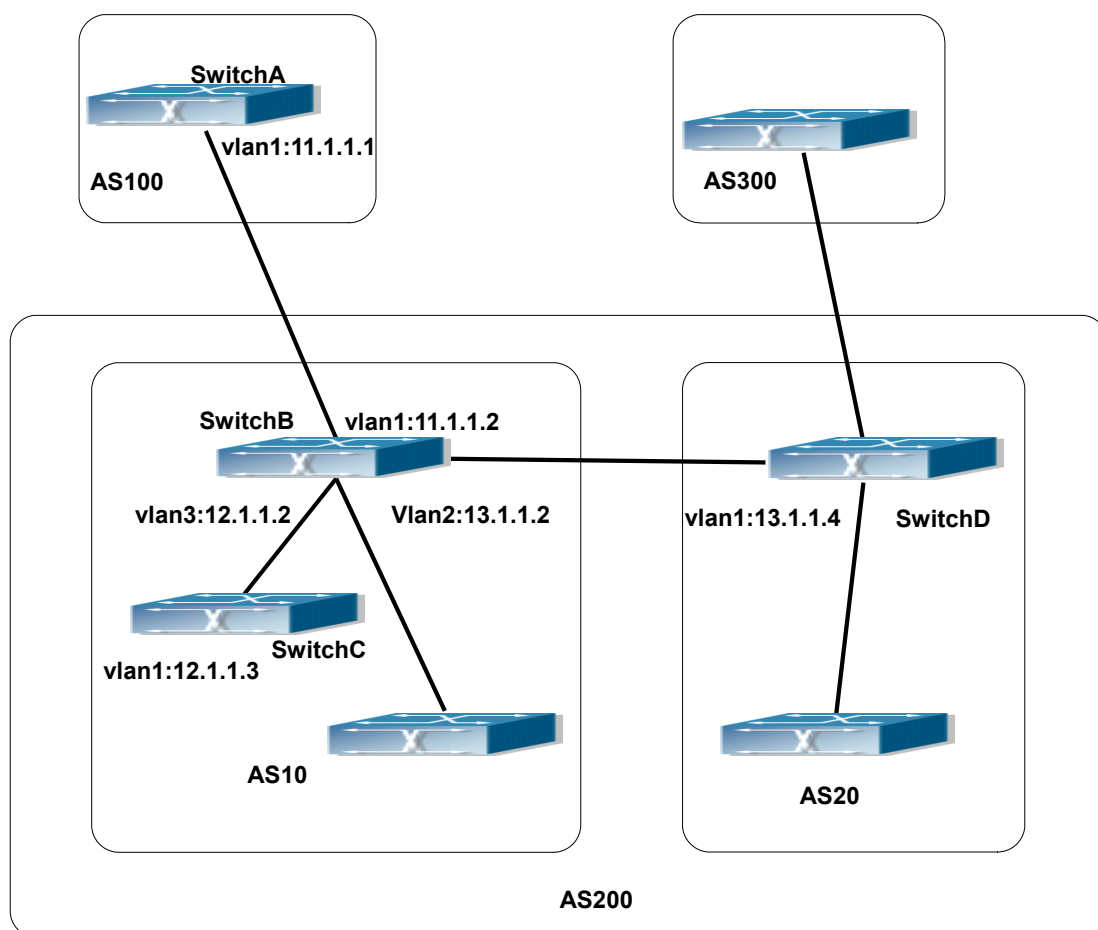
Figure 39-3-2 Confederation configuring topology
