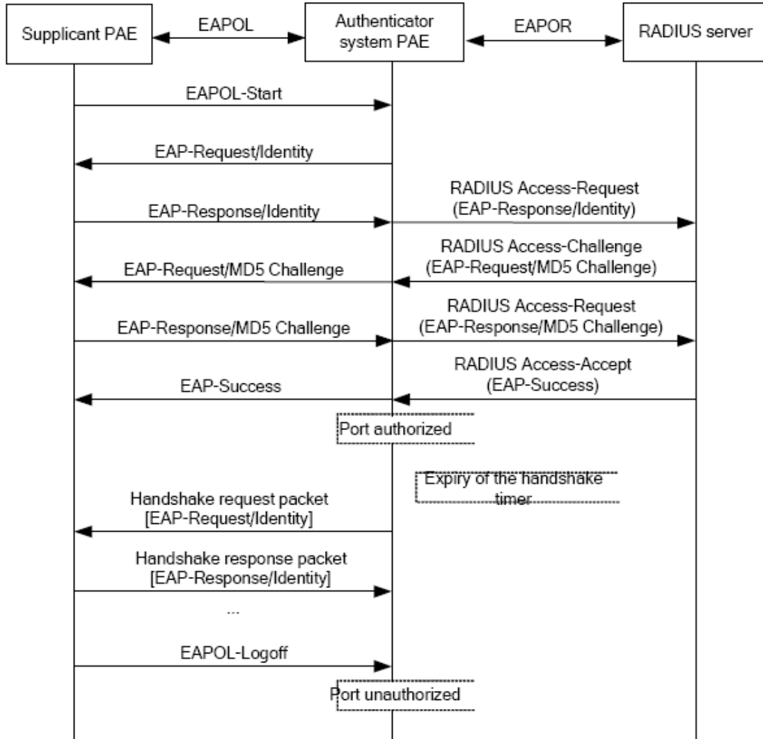
Figure 47-1-9 the Authentication Flow of 802.1x EAP-MD5
