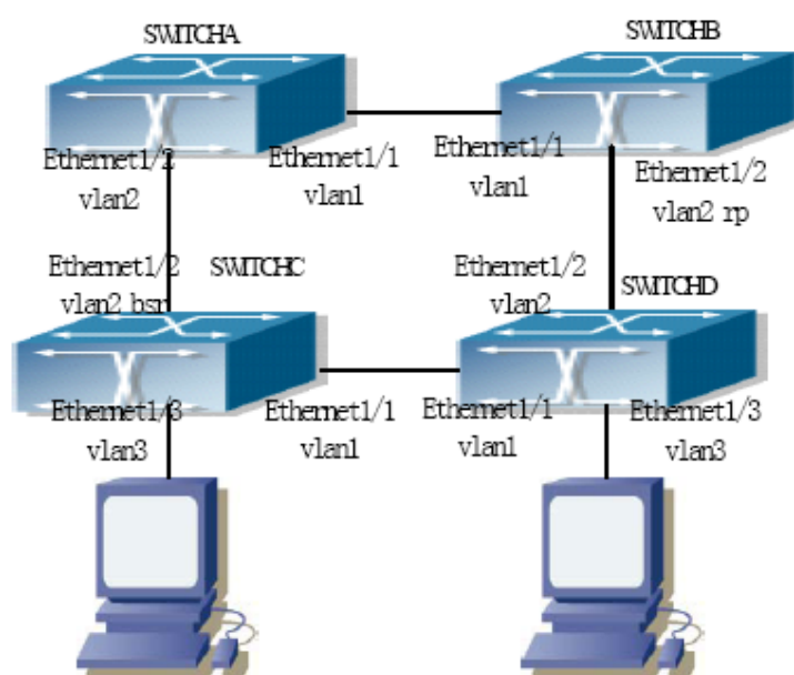
Figure 46-3-1 PIM-SSM typical environment
