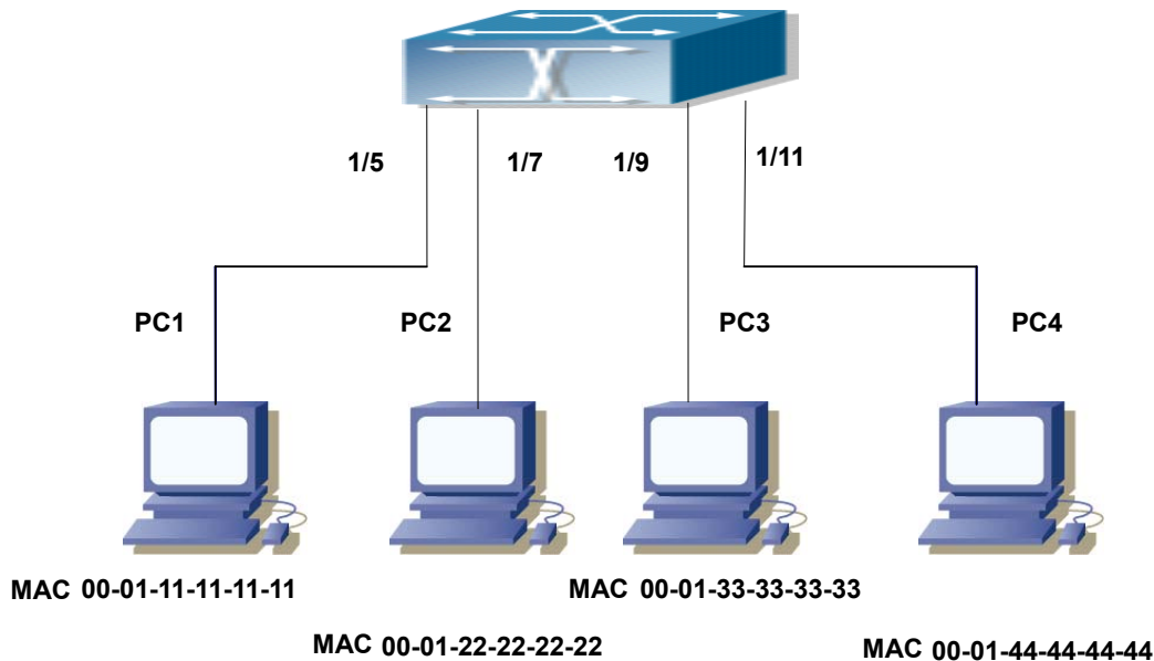
Figure 15-3-1 MAC Table typical configuration example
