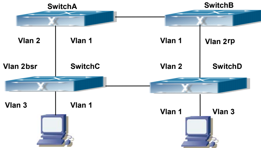
Figure 43-3-1 PIM-SM Typical Environment
