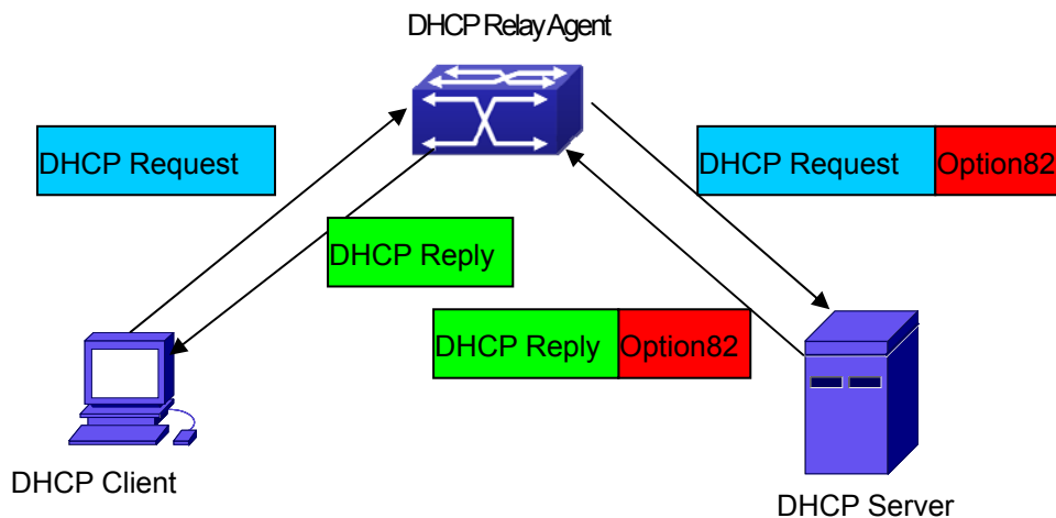
Figure 30-1-1 DHCP option 82 flow chart
