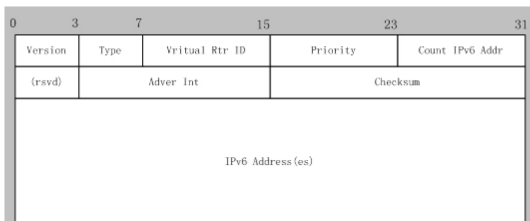
Figure 59-1-1 VRRPv3 message
