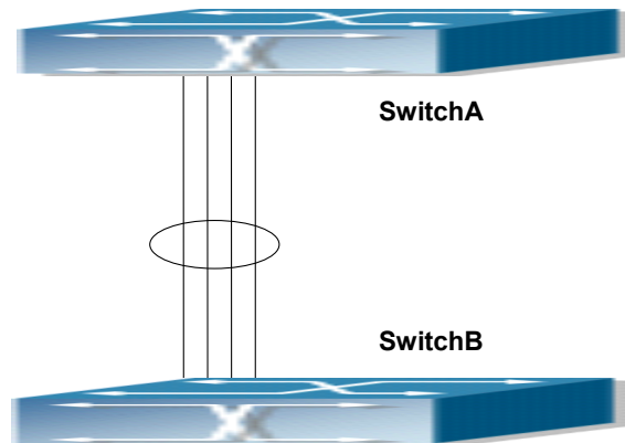
Figure 12-4-2 Configuring Port Channel in ON mode
