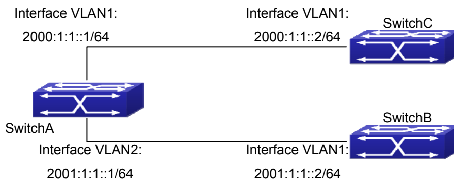
Figure 36-3-1 RIPng Example
