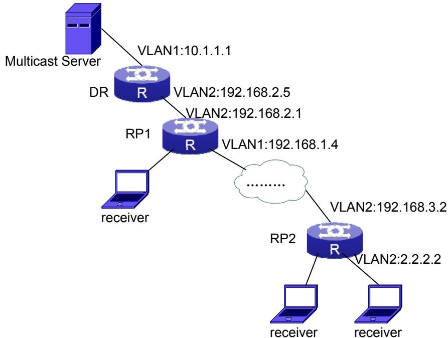
Figure 43-5-1 The ANYCAST RP v4 function of the router
