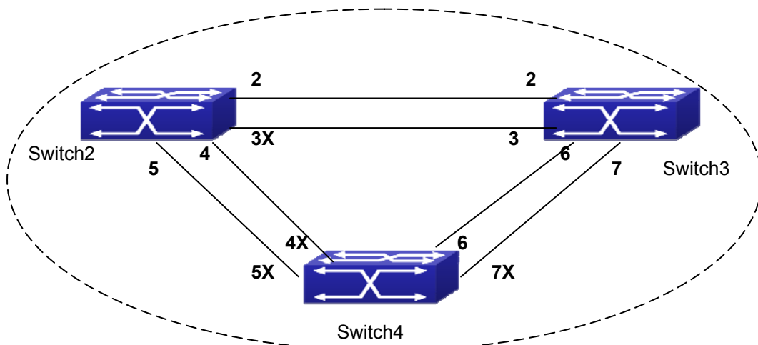
Figure 16-3-3 The Topology Of the Instance 3 after the MSTP Calculation
