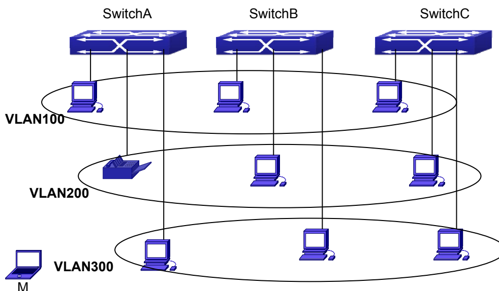
Figure 14-5-1 Typical topology application of dynamic VLAN
