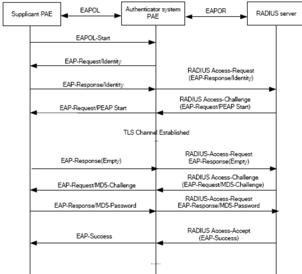
Figure 47-1-11 the Authentication Flow of 802.1x PEAP
