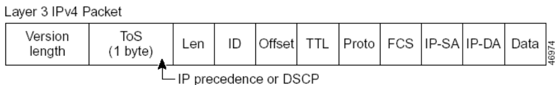
Figure 17-1-2 ToS priority
