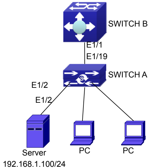
Figure 22-3-1 ARP scanning prevention typical configuration example
