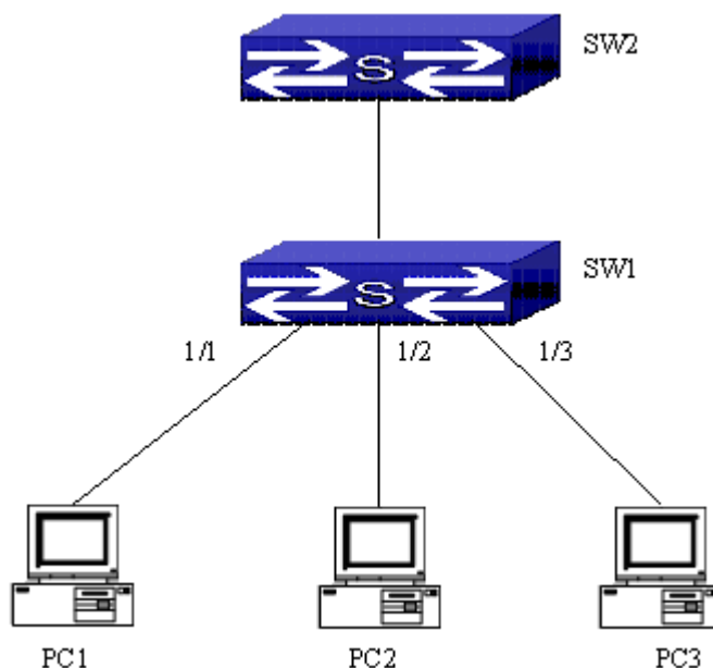
Figure 27-3-1 ND Snooping typical configuration
