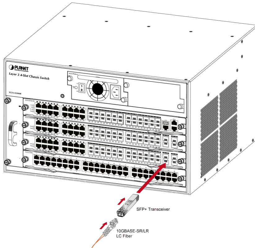
Figure 2-2-10 Plug-in the SFP+ transceiver
