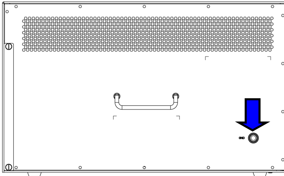
Figure 2-2-4 grounding posts
