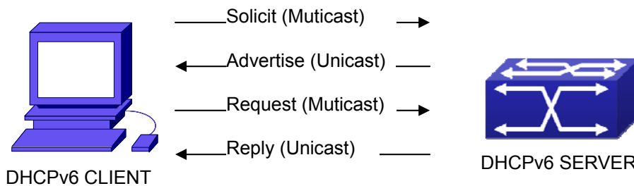
Figure 29-1-1 DHCPv6 negotiation
