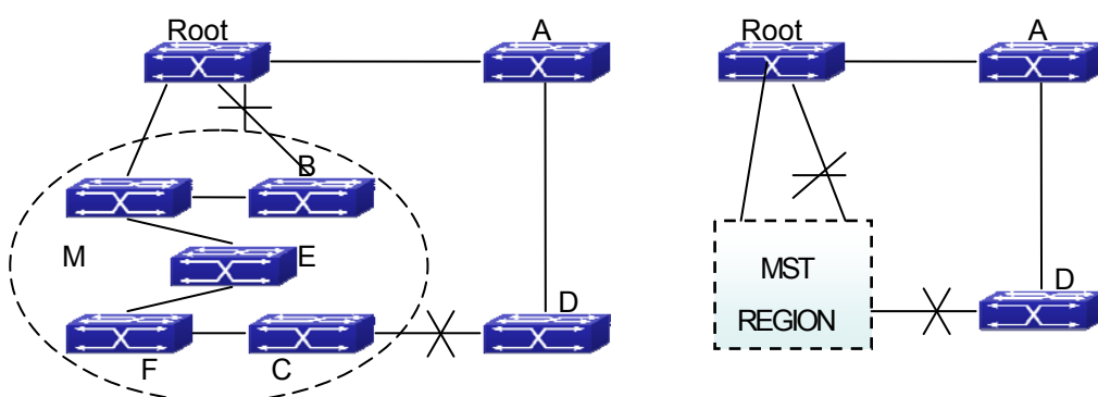
Figure 16-1-1 Example of CIST and MST Region
