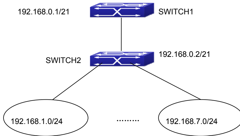
Figure 41-4-1 IPv4 Black Hole Routing Configuration Example
