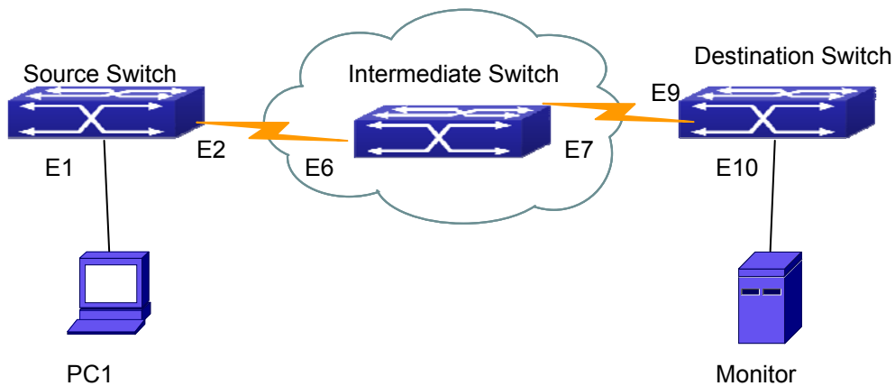
Figure 56-3-1 RSPAN Application Sample
