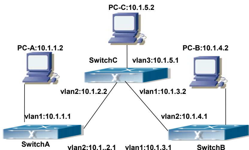
Figure 34-4-1 Static Route Configurations
