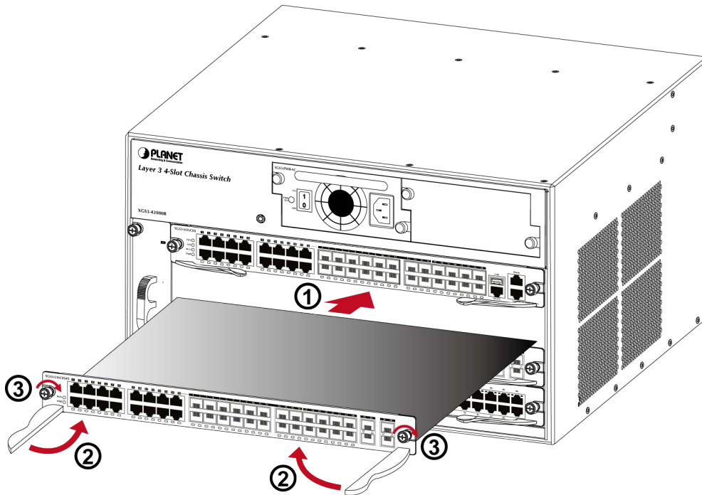
Figure 2-2-5 Insert the optional module into the slot of XGS3-42000R
