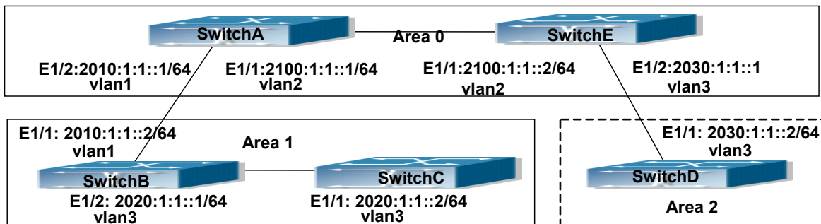
Figure 38-3-1 Network topology of OSPF autonomous system
