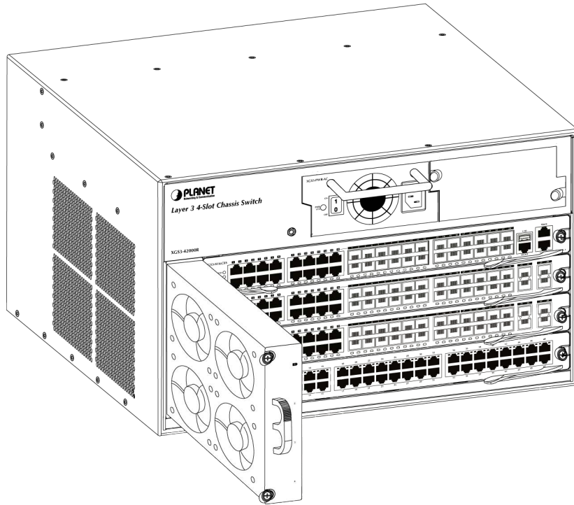
Figure 2-2-7 Installation and Removal the Fan Tray
