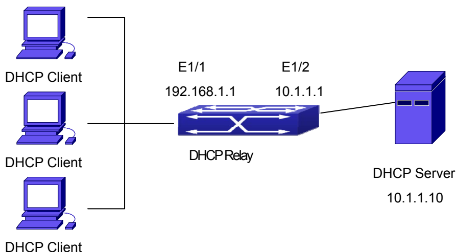
Figure 28-4-1 DHCP Relay Configuration
