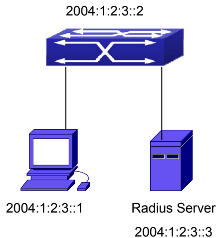
Figure 47-3-4 IPv6 Radius
