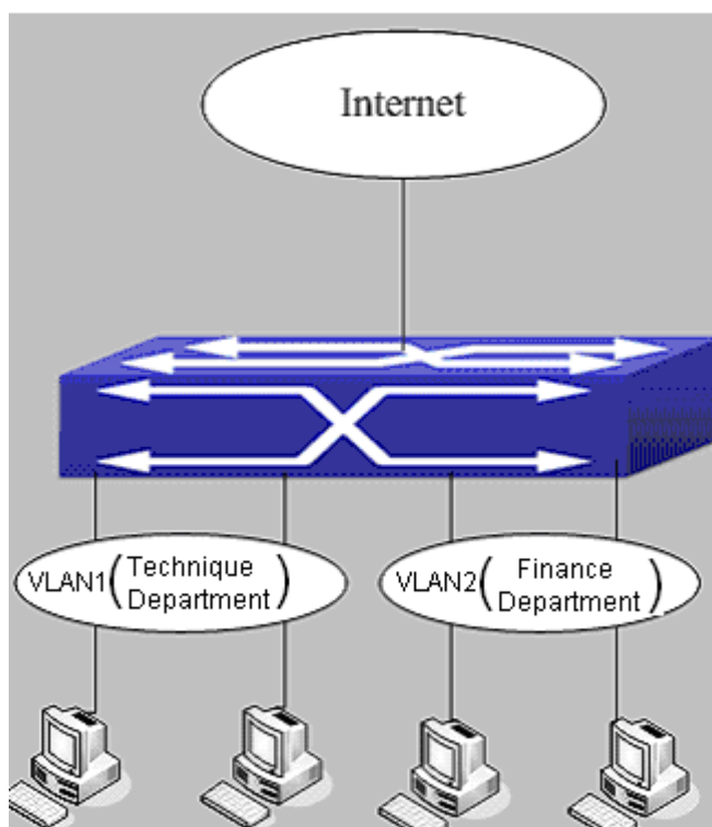
Figure 55-3-1 VLAN-ACL configuration example
