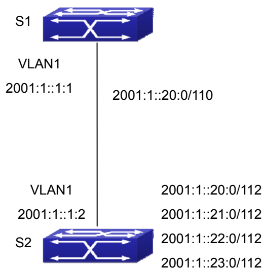
Figure 36-3-2 Typical application of RIPng aggregation
