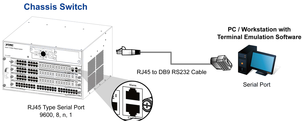
Figure 3-1-1 Out-of-band Management Configuration Environment
