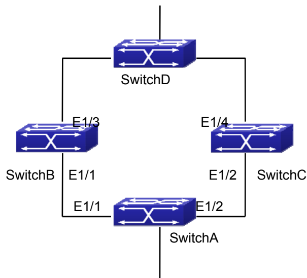
Figure 62-3-1 ULSM typical example
