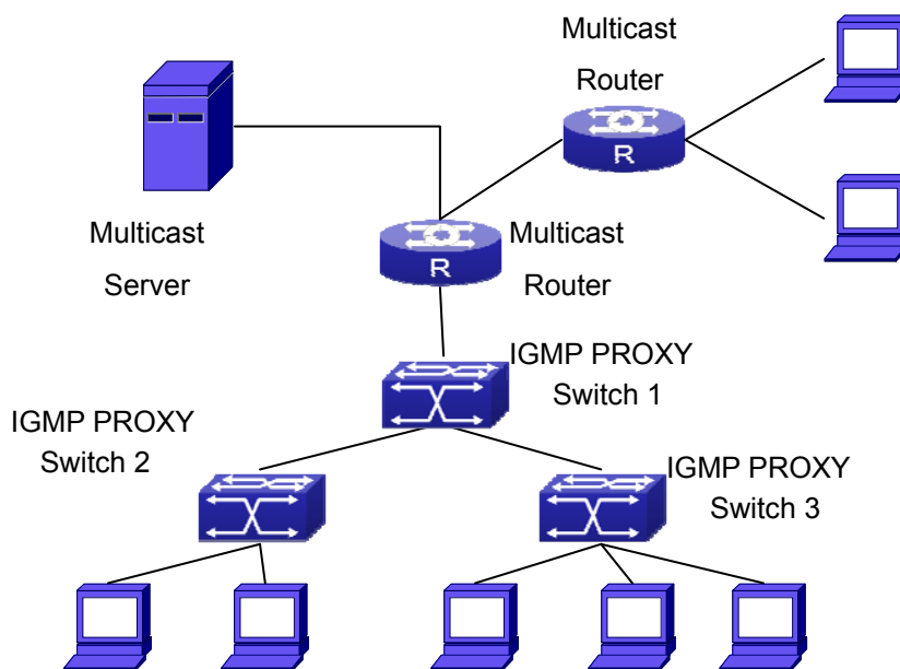
Figure 43-11-1 IGMP Proxy Topology Diagram
