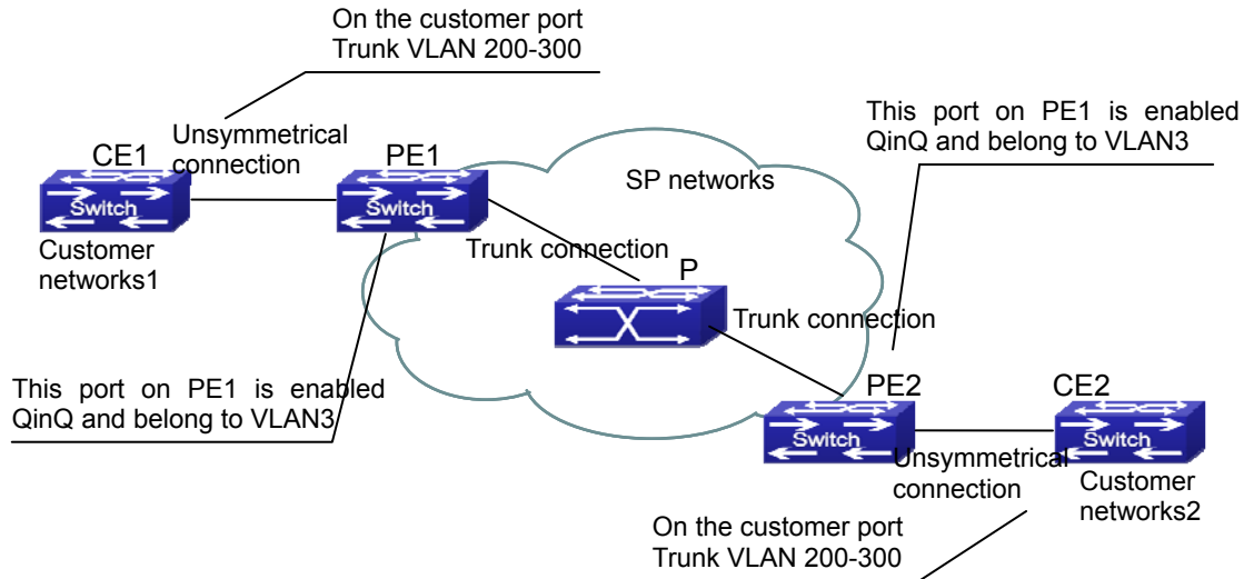
Figure 14-4-1 Vlan translation topology mode
