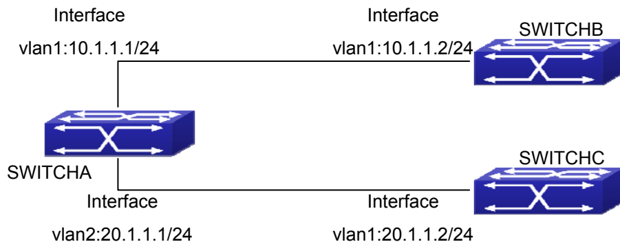
Figure 37-3-4 OSPF VPN Example
