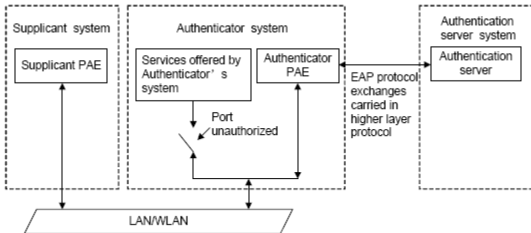
Figure 47-1-1 The Authentication Structure of 802.1x
