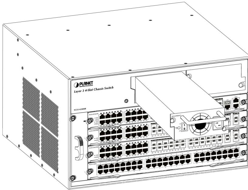
Figure 2-2-8 Install and Removal the Power Supply Unit
