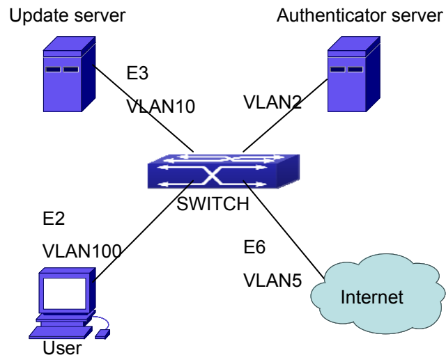
Figure 47-3-1 The Network Topology of Guest VLAN
