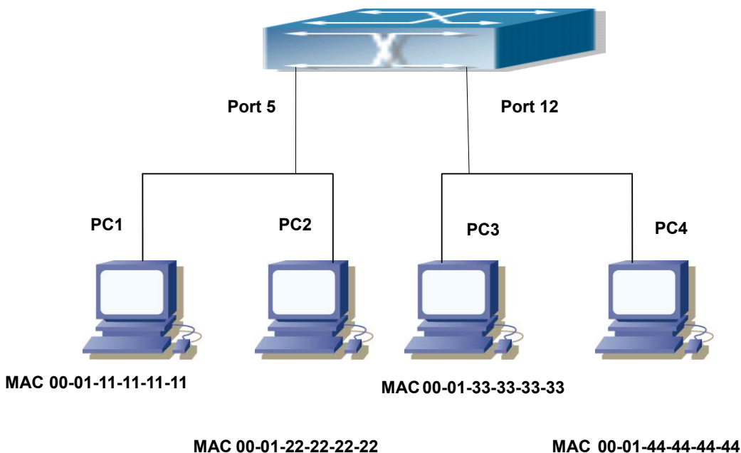
Figure 15-1-1 MAC Table dynamic learning
