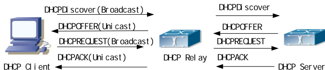
Figure 28-3-1 DHCP relay
