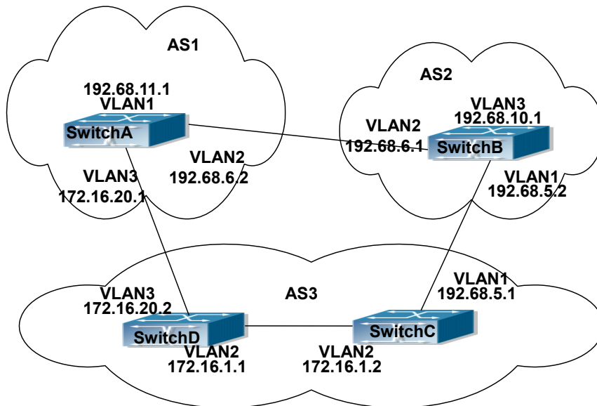
Figure 33-2-1 Policy routing Configuration
