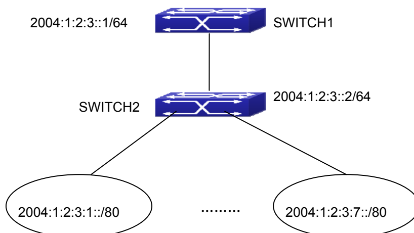
Figure 41-4-2 IPv6 Black Hole Routing Configuration Example
