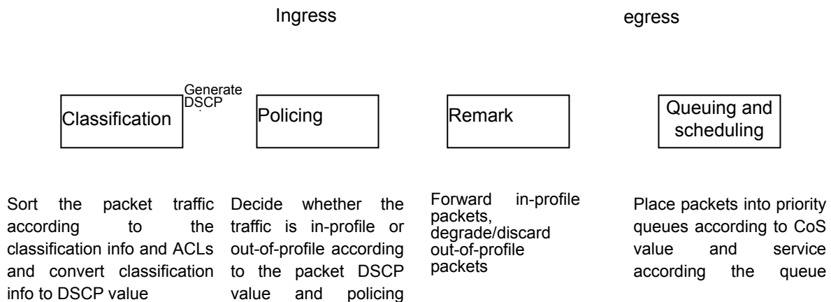
Figure 17-1-3 Basic QoS Model
