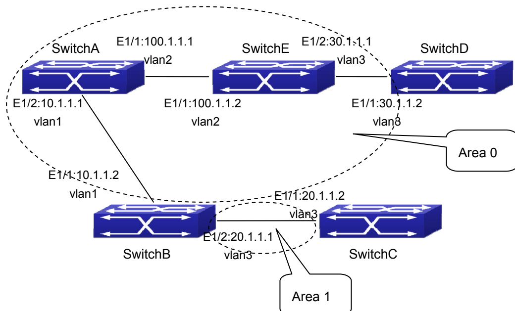
Figure 37-3-1 Network topology of OSPF autonomous system
