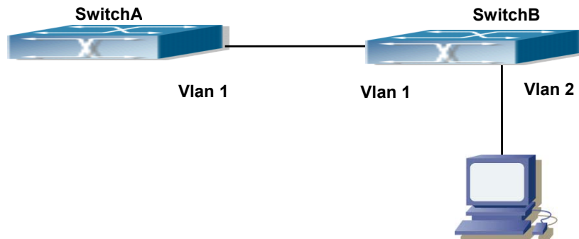
Figure 43-7-1 DVMRP Network Topology Diagram
