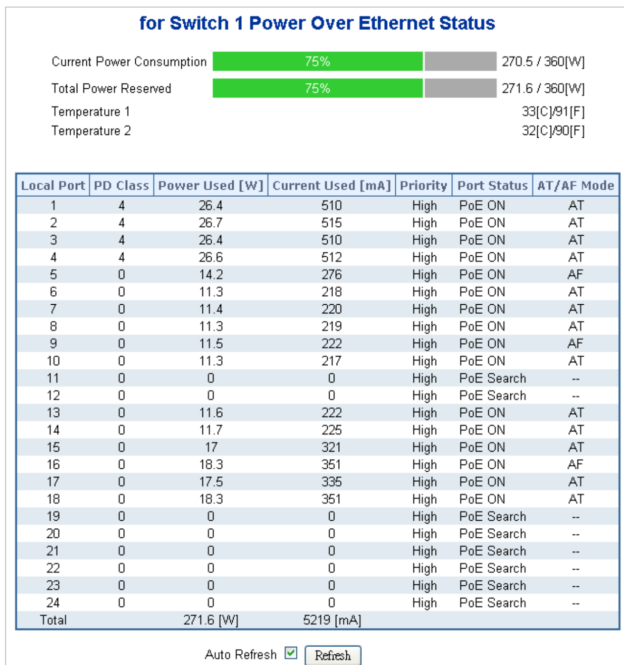
Figure 4-16-4 PoE Status screenshot
