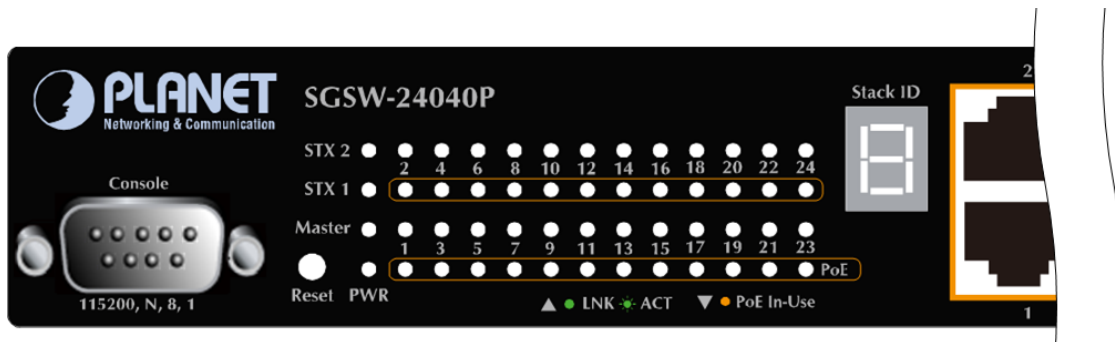
Figure 2-5 SGSW-24040P / SGSW-24040P4 LED panel
