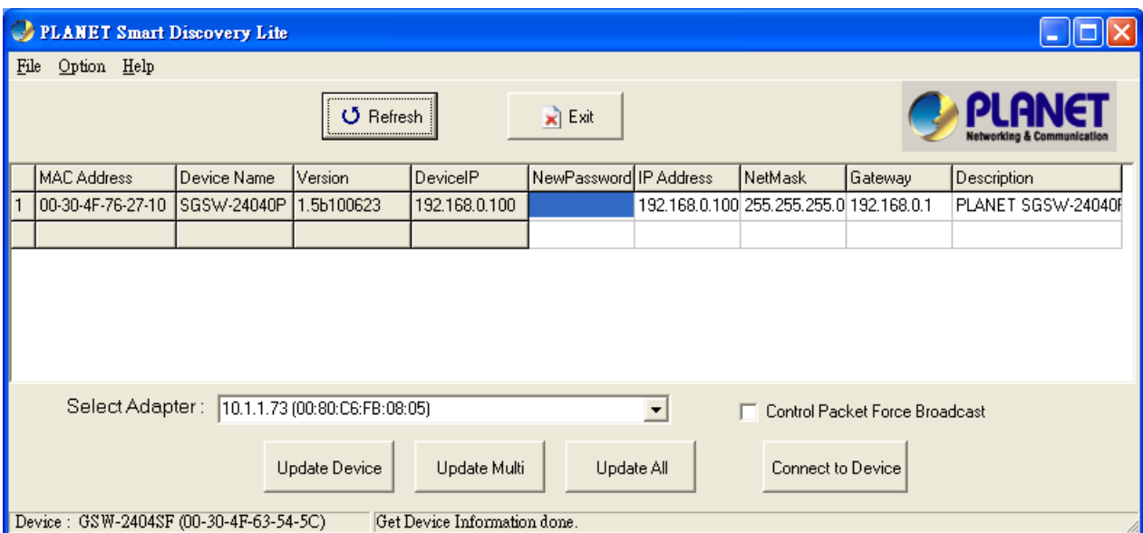
Figure 2-24 Use PLANET Smart Discovery Utility to display the IP address of stack master
