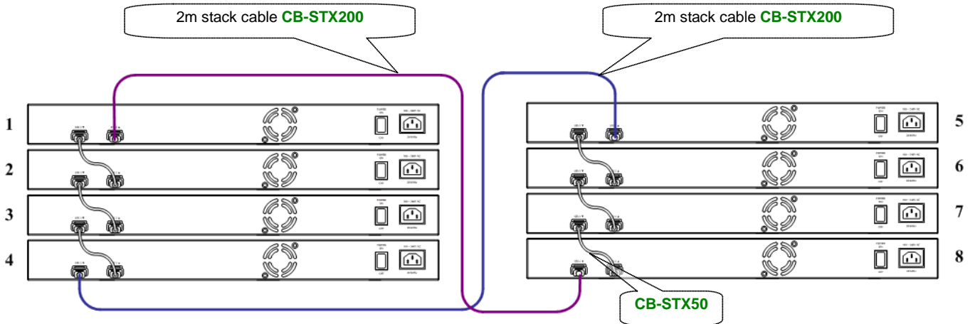
Figure 2-25 Separated Stack connection
