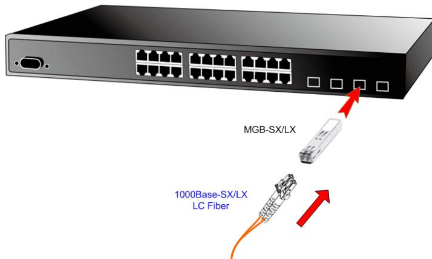
Figure 2-17 Plug-in the SFP transceiver
