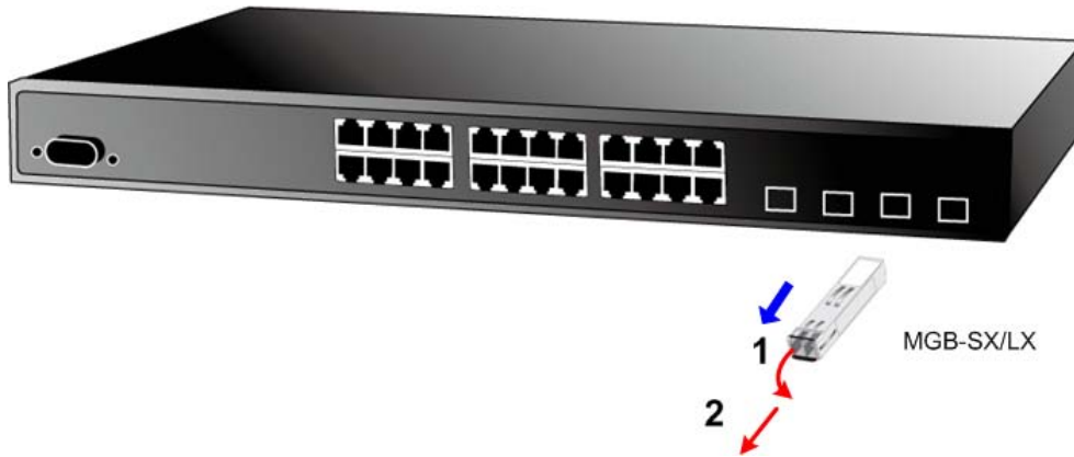
Figure 2-18 Pull out the SFP transceiver
