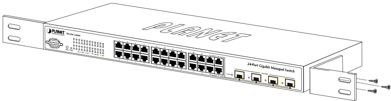
Figure 2-15 Attach brackets to the Managed Switch.
