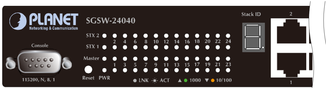
Figure 2-4 SGSW-24040 / SGSW-24040R LED panel
