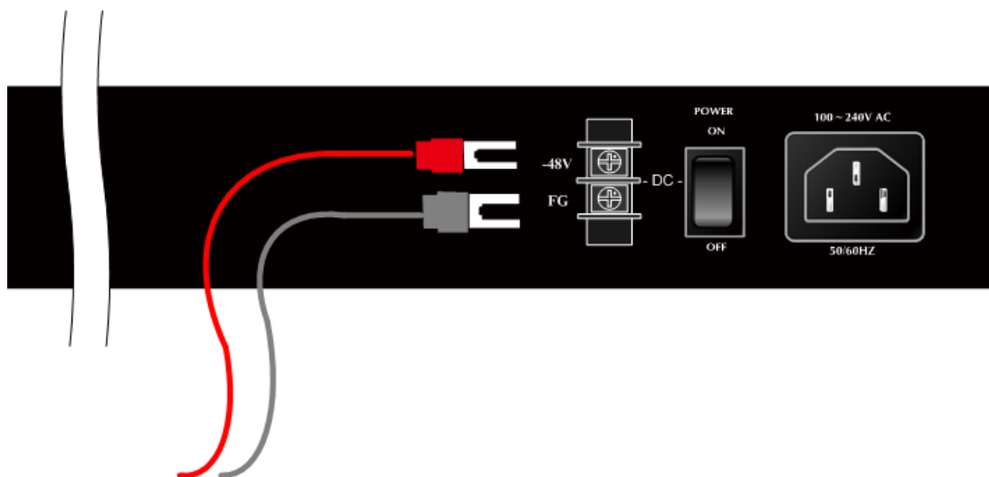
Figure 2-19 -48VDC connector
