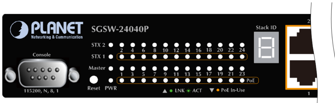
Figure 2-5 SGSW-24040P / SGSW-24040P4 LED panel
