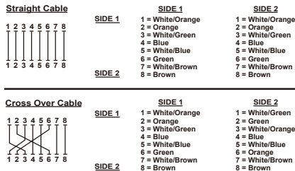
Figure A-1: Straight-Through and Crossover Cable
