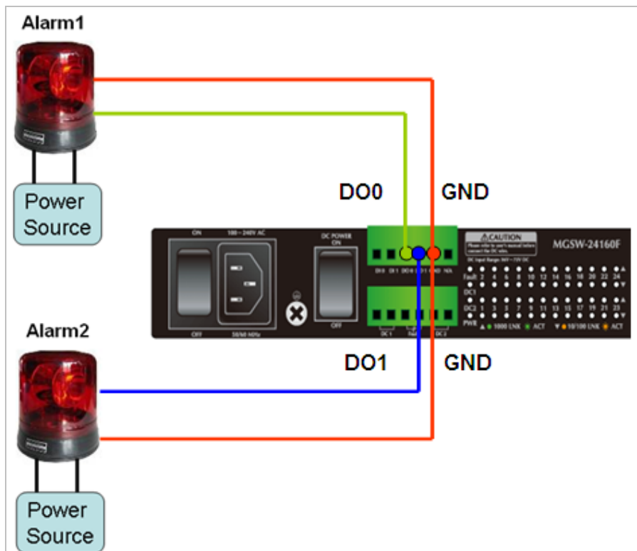
Figure 2-14 Wires DO0 and DO1 to Open Detector
