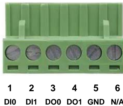
Figure 2-12 6-Pin Terminal Block DI / DO Wiring Input
