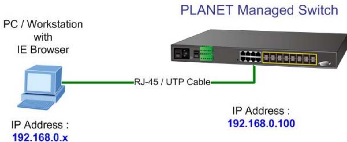
Figure 4-1-1 Web Management Diagram
