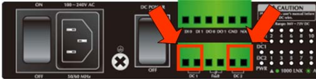
Figure 2-9 Wiring the Redundant Power Inputs
