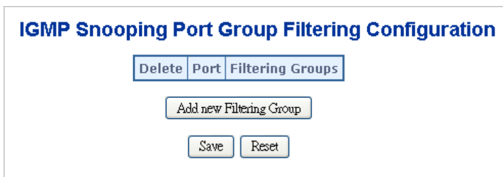
Figure 4-8-8 IGMP Snooping Port Group Filtering Configuration Page Screenshot
