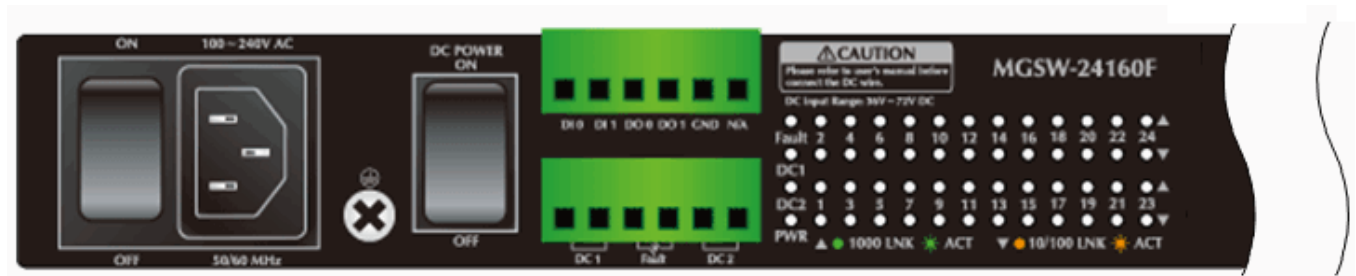
Figure 2-2 MGSW-24160F LED Panel
