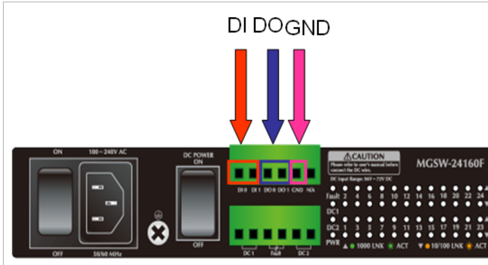
Figure 2-11 Wiring the Redundant Power Inputs
