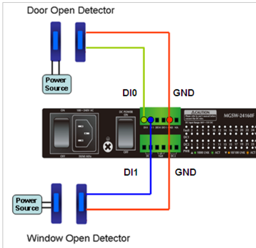
Figure 2-13 Wires DI0 and DI1 to Open Detector
