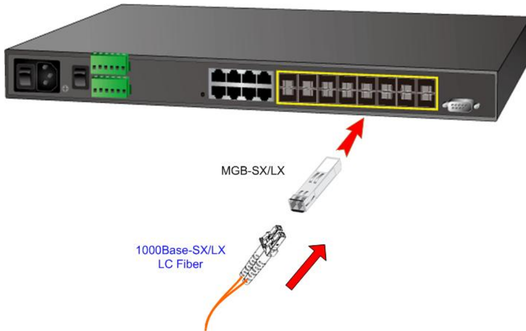
Figure 2-7 Plug-in the SFP Transceiver
