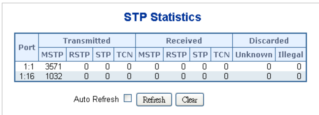
Figure 4-7-12 STP Statistics Page Screenshot
