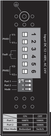
Figure 2-2: Industrial Gigabit Media Converter Upper Panel
