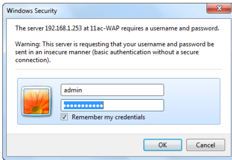
Figure 4-6 Login Window
