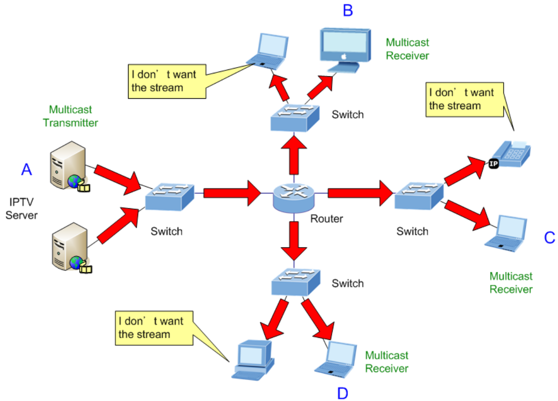
Figure 4-12-2 Multicast Flooding
