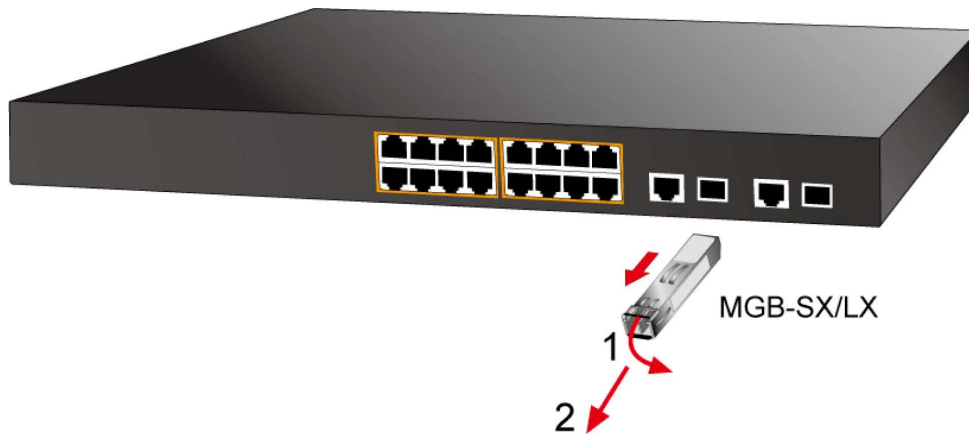
Figure 2-8 How to Pull Out the SFP Transceiver
