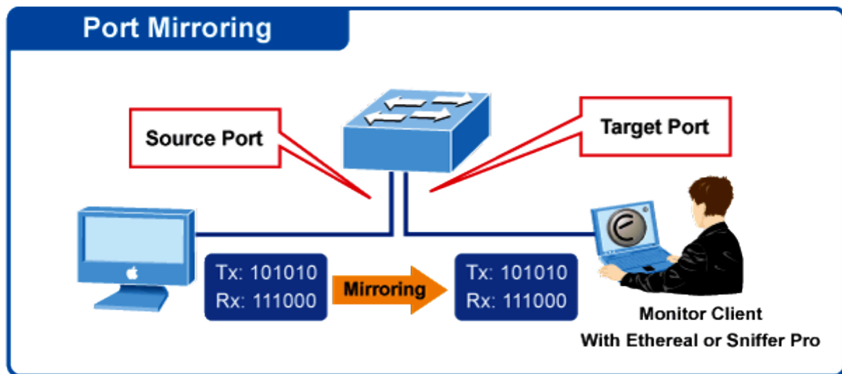
Figure 4-3-8 Port Mirror Application
