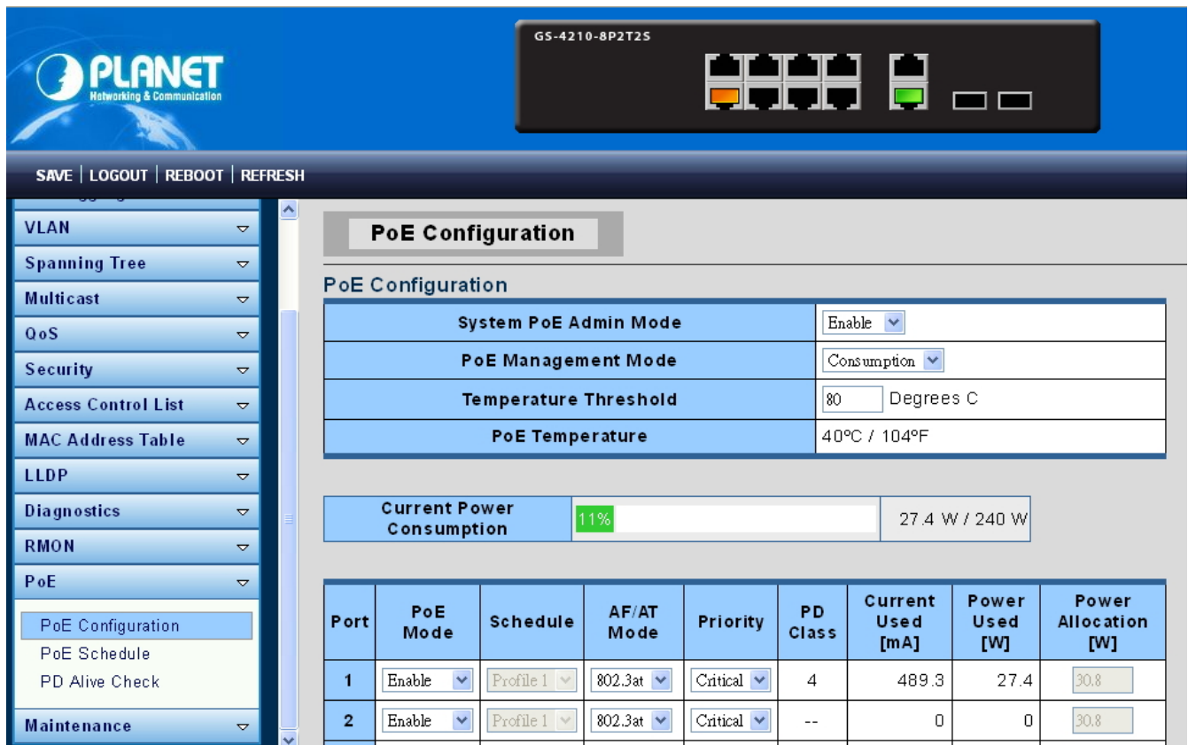
Figure 4-16-1: Power over Ethernet Status
