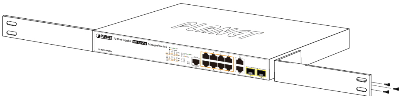
Figure 2-1-5 Attach Brackets to the Managed Switch.
