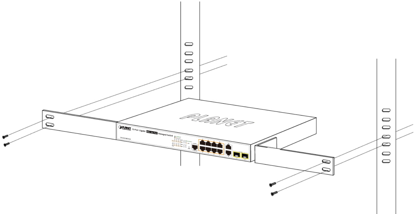
Figure 2-1-6 Mounting Managed Switch in a Rack
