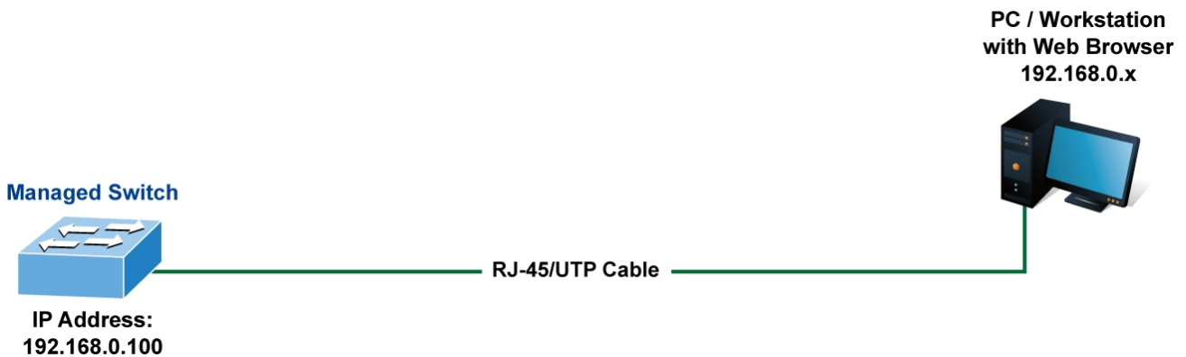
Figure 3-1-3: Web Management
