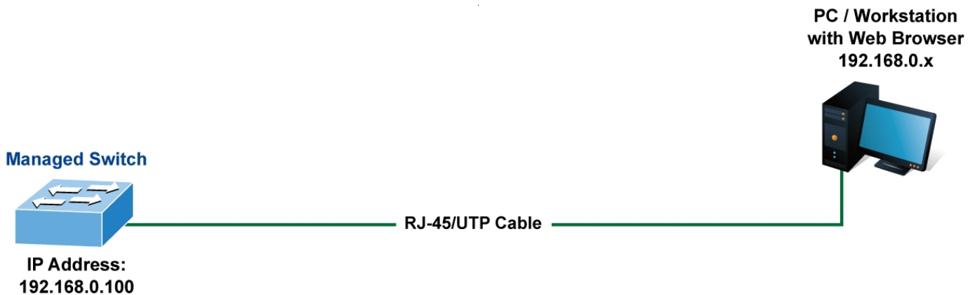
Figure 4-1-1: Web Management
