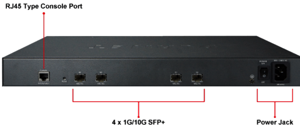
Figure 2-1-3: Rear Panel of GS-5220-48T4X
