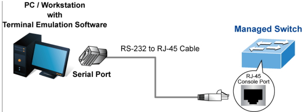
Figure 3-1-1: Console Management
