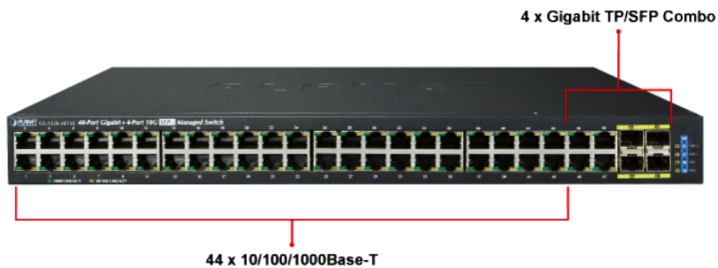
Figure 2-1-1: Front Panel of GS-5220-48T4X
