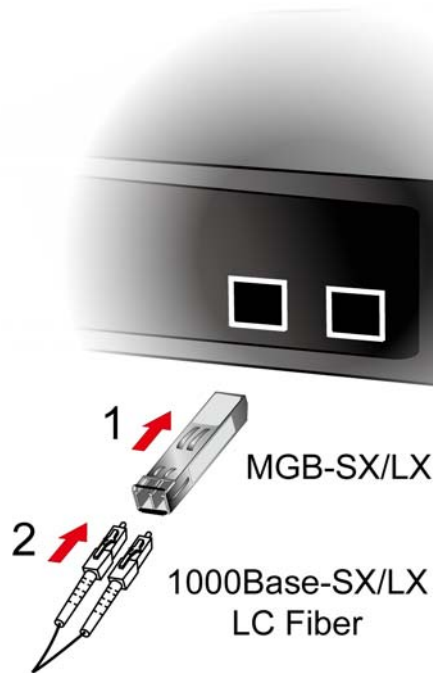
Figure 2-2-4: Plug-in the SFP/SFP+ Transceiver
