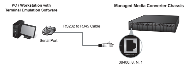
Figure 4-1: Managed Media Converter Chassis Console Connectivity
