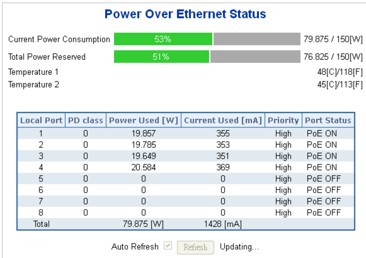
Figure 4-16-4 PoE Status screenshot
