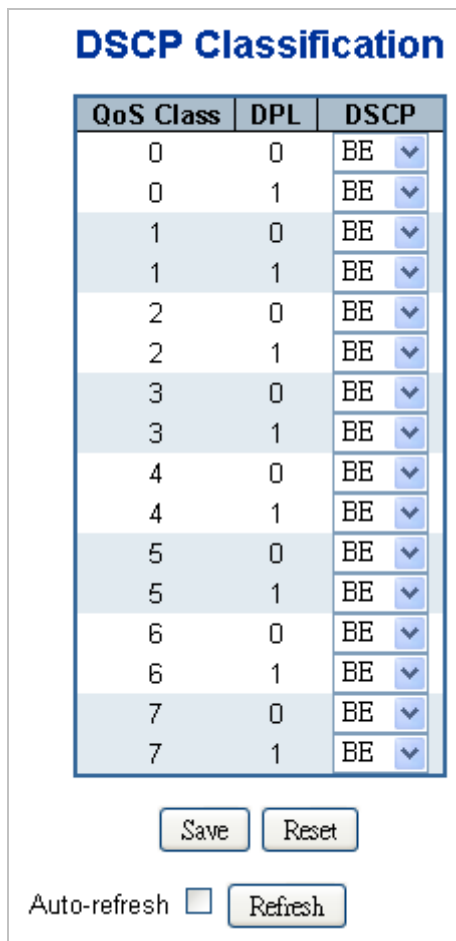
Figure 4-9-12 DSCP Classification page screenshot
