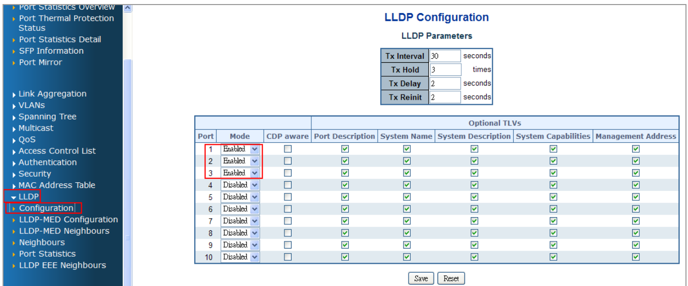
Figure 4-16-7 LLDP Configuration screenshot
