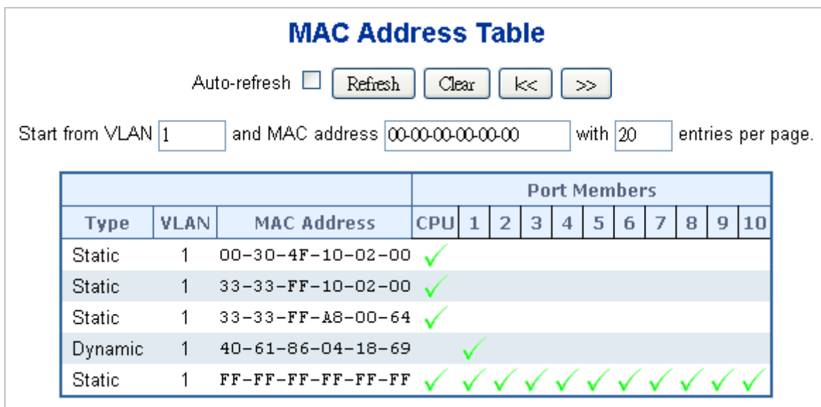
Figure 4-13-2 MAC Address Table Status
