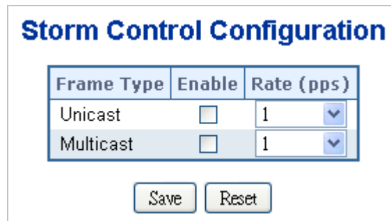
Figure 4-9-16 Storm Control Configuration page screenshot
