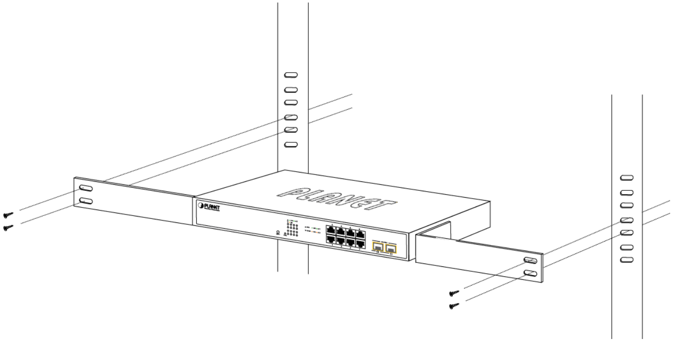
Figure 2-9 Mounting WGSD-10020 in a Rack
