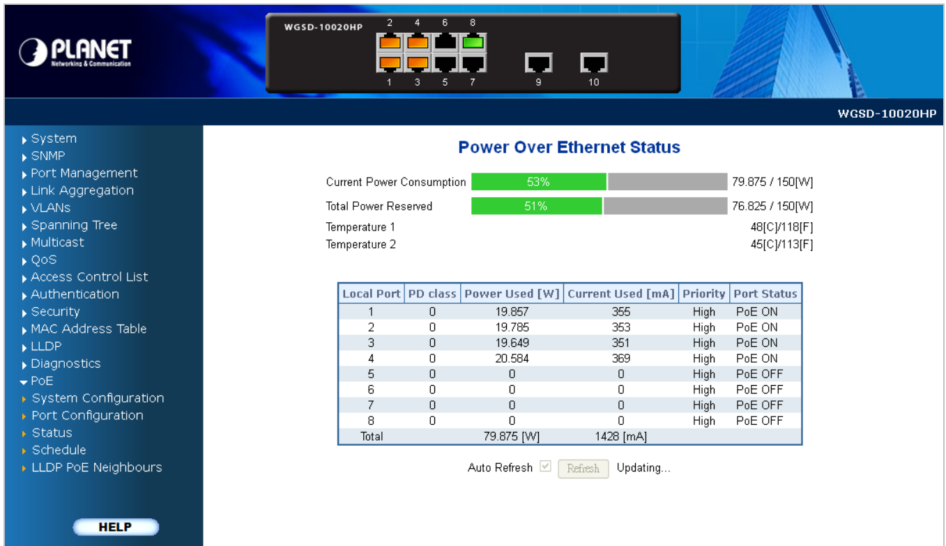
Figure 4-16-1 Power over Ethernet Status
