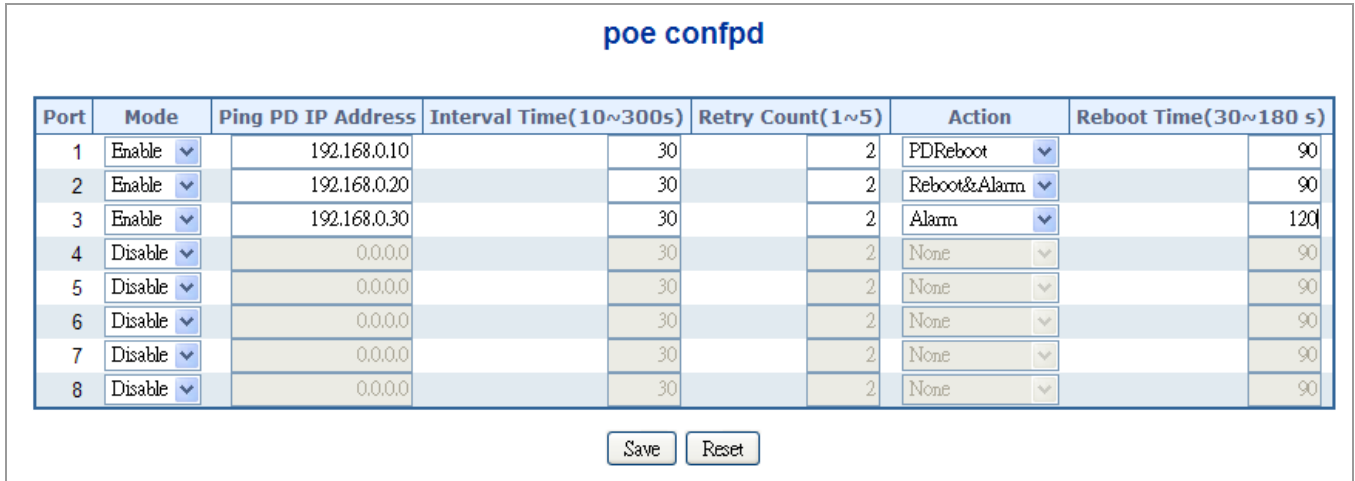
Figure 4-16-8 PD Alive CCheck Configuration screenshot
