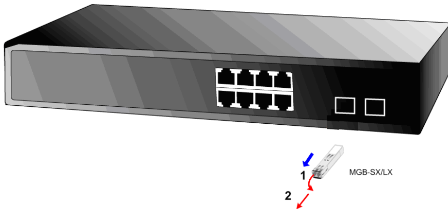
Figure 2-11 Pull out the SFP transceiver
