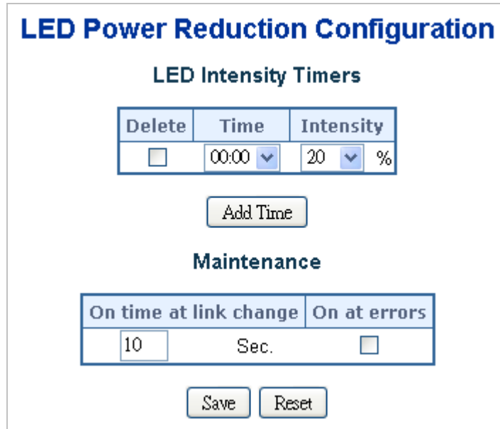
Figure 4-2-17 LED Power Reduction page screenshot
