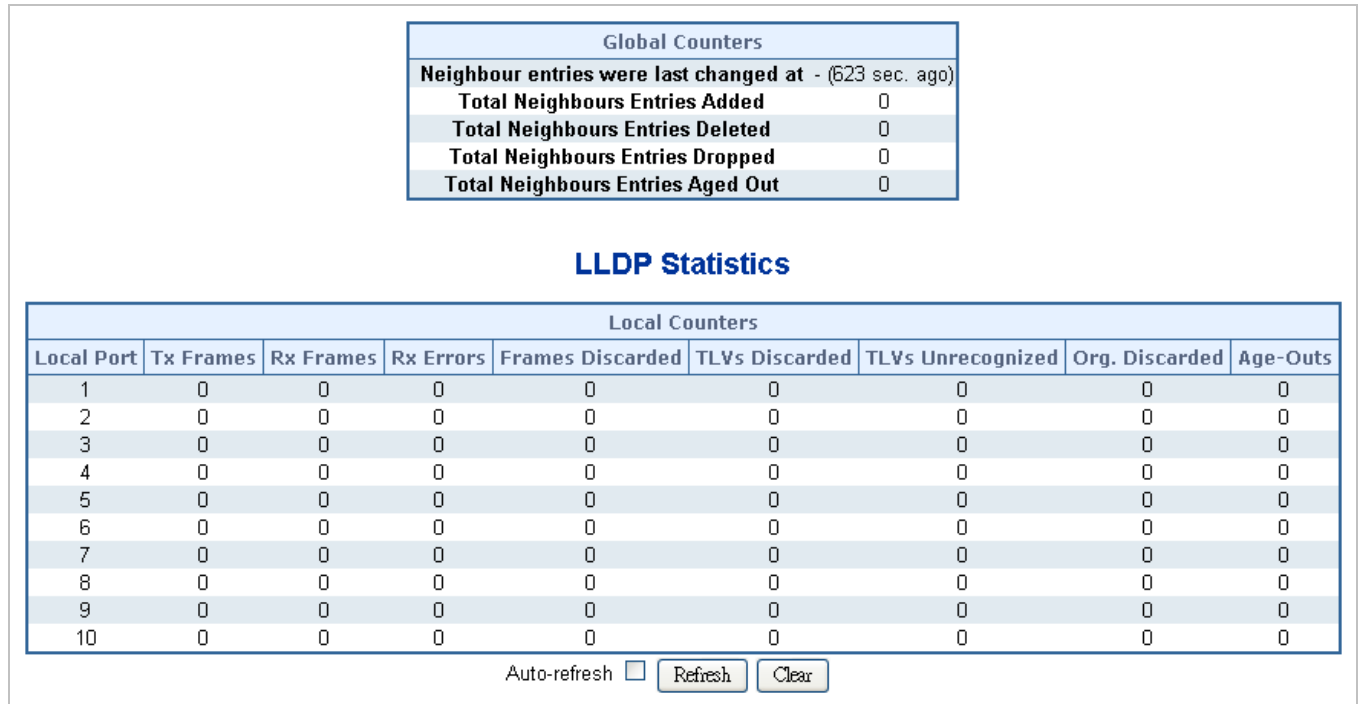
Figure 4-14-5 LLDP Statistics page screenshot
