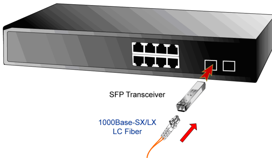
Figure 2-10 Plug-in the SFP transceiver
