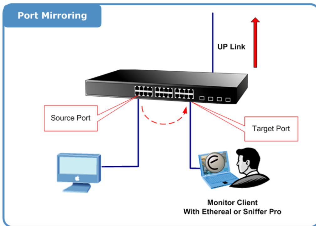
Figure 4-4-6 Port Mirror application
