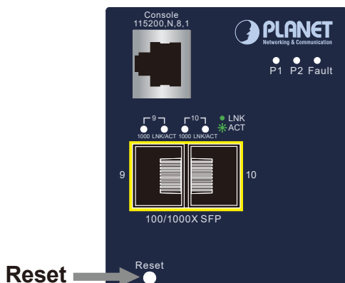
Figure 6-1: IGS-4215-4P4T/IGS-4215-4P4T2S Reset Button
