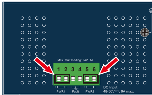
Figure 3-2: IGS-4215-8P2T2S DC Inlet Power Socket
