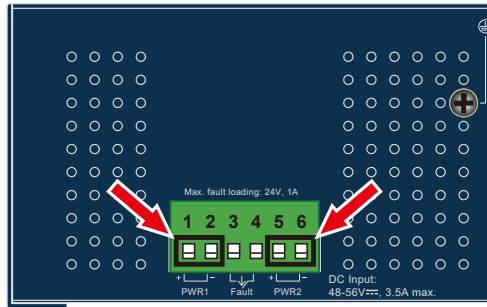
Figure 3-1: IGS-4215-4P4T/IGS-4215-4P4T2S DC Inlet Power Socket
