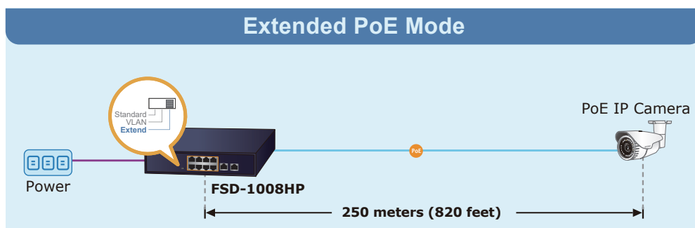
10BASE-T UTP with PoE
