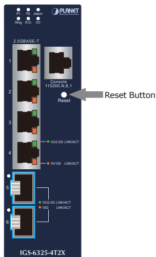
Figure 6-2: IGS-6325-4T2X Reset Button
