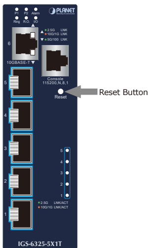
Figure 6-1: IGS-6325-5X1T Reset Button
