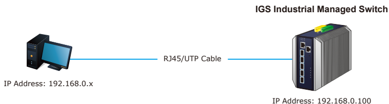
Figure 5-1: IP Management Diagram
