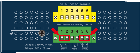
Figure 3-1: IGS-6325-5X1T Upper Panel
