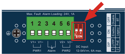
Figure 2-2: IGUP-805AT Upper Panel
